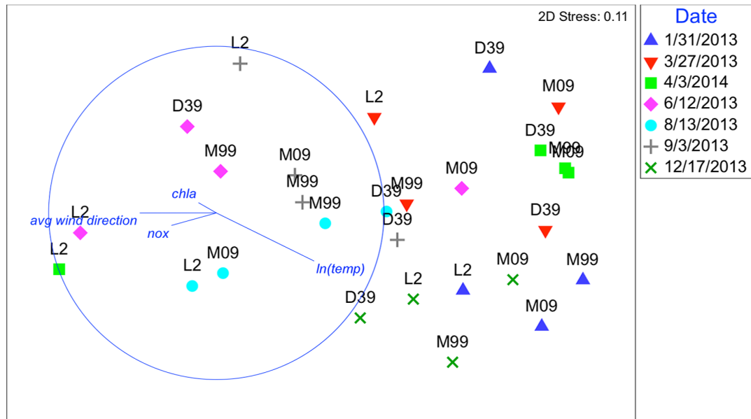
FIGURE 5 | Nonmetric multidimensional scaling (NMDS): plot of 28 biological samples, coded by date and station with best explanatory environmental variable overlay. Data represent sequence relative abundances; resemblances based on Bray–Curtis similarity. Plots are overlaid with best explanatory environmental variable vectors, pointing in the direction of increasing \ln(\text{temp}) , chl a , NO x , and weekly average wind direction. The length of the vectors shows the strength of the relationship.
