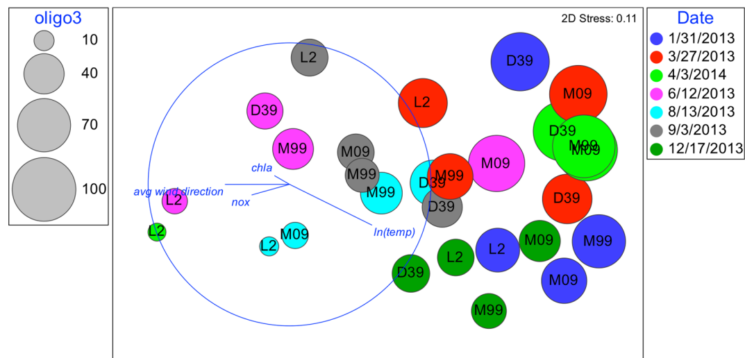
FIGURE 6 | Nonmetric multidimensional scaling: plot of 28 biological samples, coded by date and station with best explanatory environmental variable overlay. Relative abundances of oligo3 are represented by the diameter of the circles.
