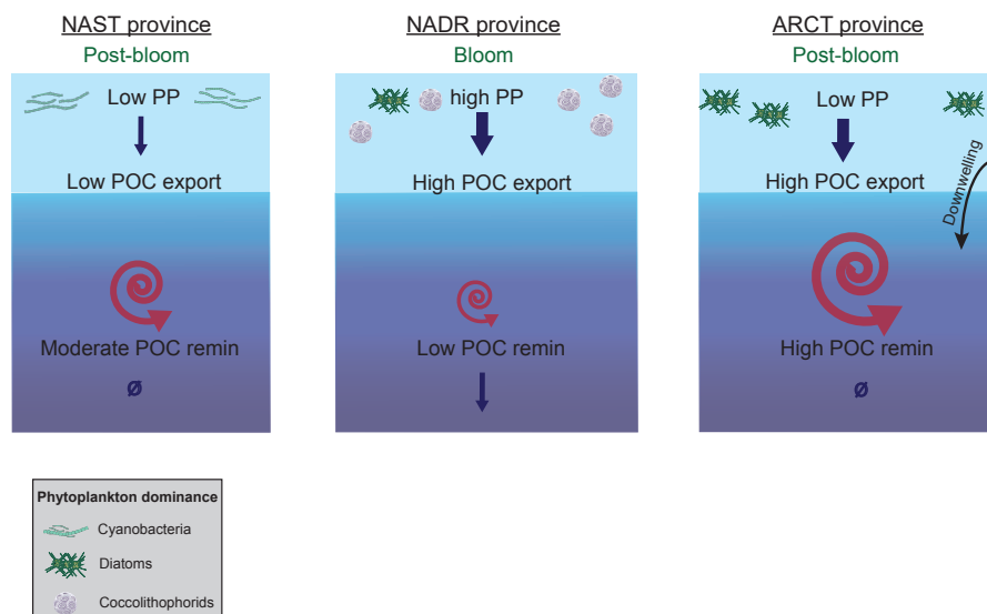
Figure 10. General schematic of the biological carbon pump in the NAST, NADR, and ARCT provinces during GEOVIDE. Primary production (PP) data from Fonseca-Batista et al. (2018; this issue) and Lemaitre et al. (2018; this issue); particulate organic carbon (POC) export fluxes from Lemaitre et al. (2018; this issue) and POC remineralisation fluxes from this study. The dominating phytoplankton communities and the stage of the bloom are also indicated.
