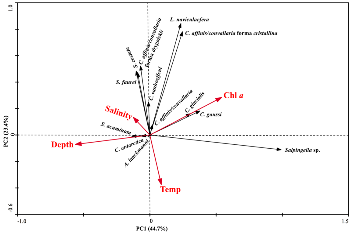
Fig. 10 Principal component analysis (PCA) of tintinnid ciliate abundance and different seawater samples associated with environmental variables. The x -axis is the first PCA axis, and the y -axis is the sec-
