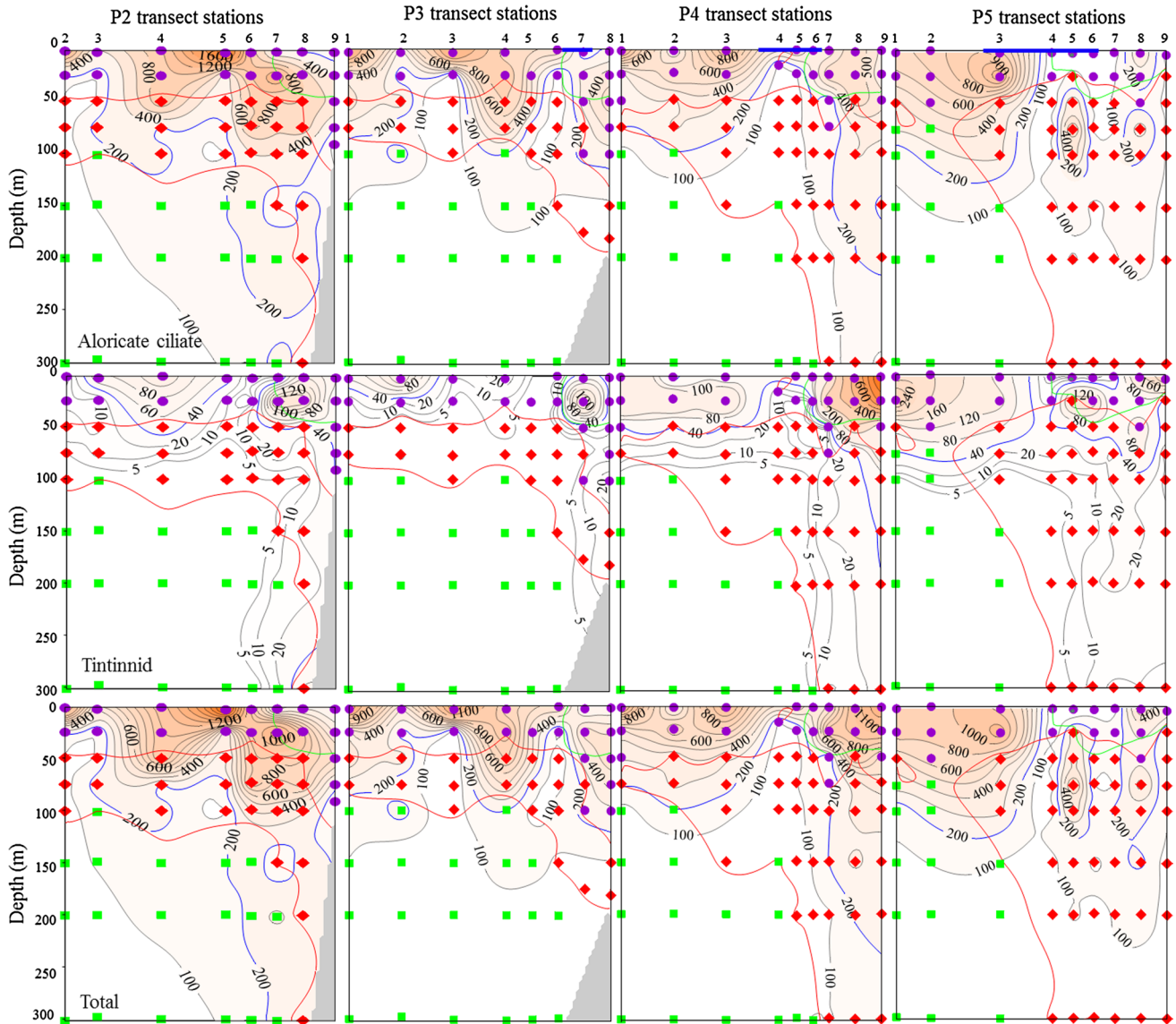
Fig. 3 Vertical distributions of abundance ( \text{ind. L}^{-1} ) of aloricate ciliate, tintinnid, and total ciliate along the transects (P2, P3, P4, P5) in open waters near Prydz Bay. Dot symbols indicate both the depths at which ciliates were sampled and the water masses where samples were attached (purple circle SSW; red diamond WW; green square
