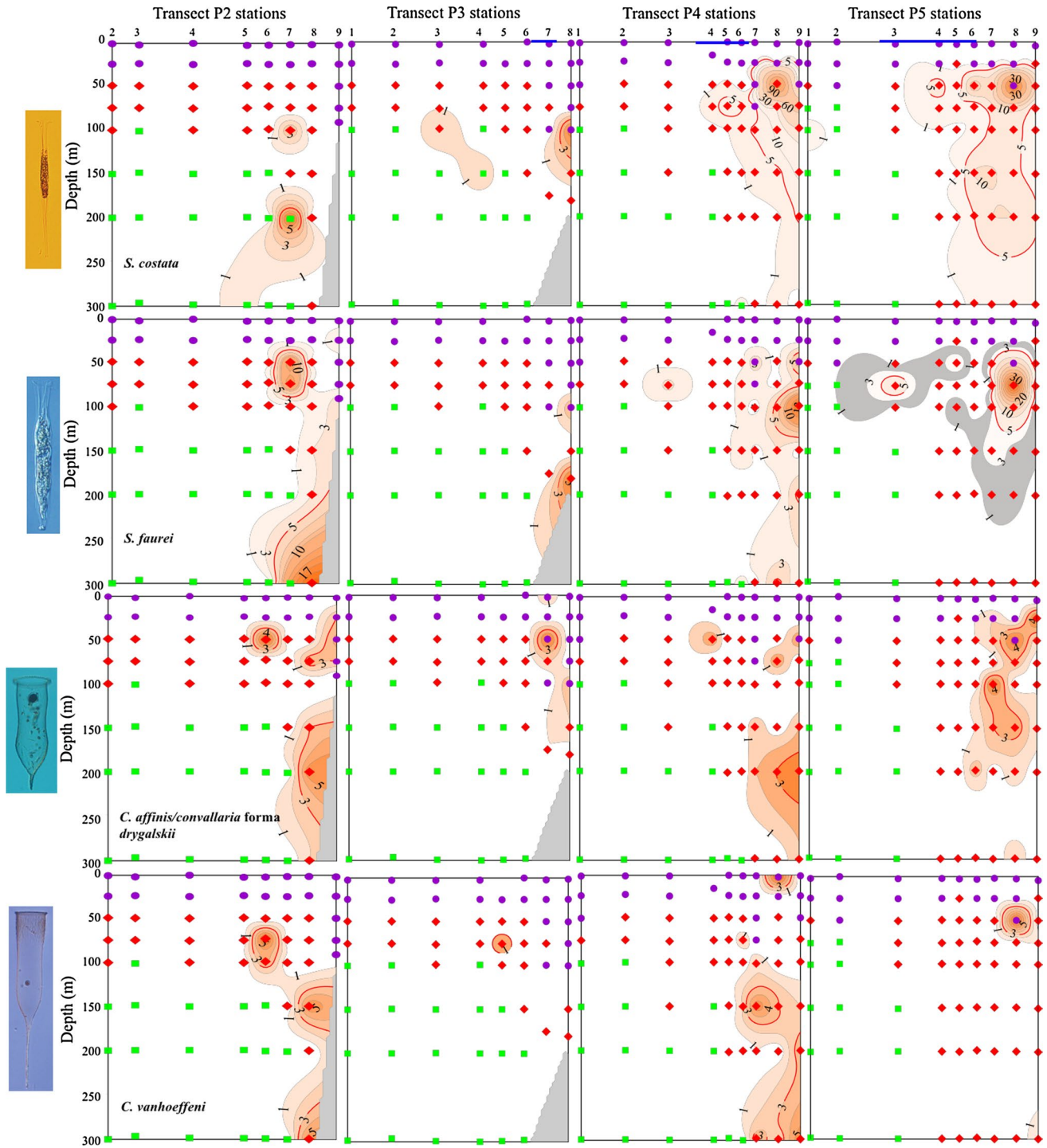
Fig. 8 Vertical distribution of abundance (ind. L -1 ) of tintinnid species (Pattern 2) in open waters near Prydz Bay. Dot symbols indicate both the depth at which ciliates were sampled and the water masses where samples were collected (purple circle SSW; red diamond WW;
