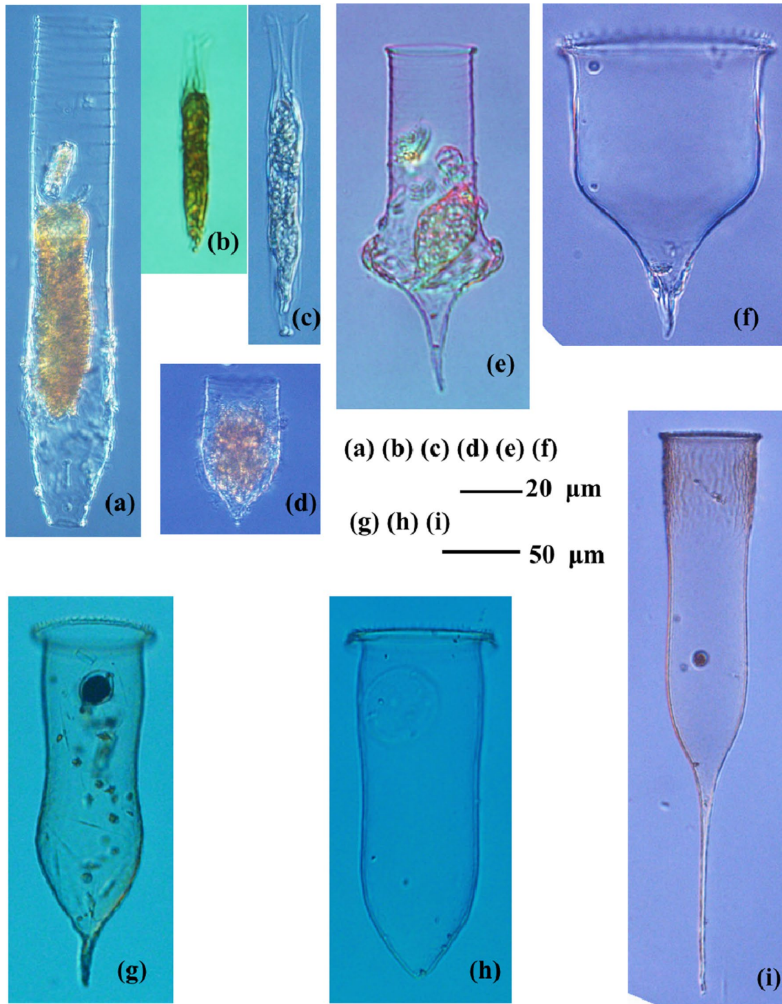
Fig. 6 Photos of some tintinnid species in open waters near Prydz Bay. a Laackmanniella naviculaefera , b Salpingella sp., c S. faurei , d Codonellopsis glacialis , e C. gaussi , f Cymatocytilis affinis/convallaria , g C. affinis/convallaria forma drygalskii , h C. affinis/convallaria forma cristallina , i C. vanhoeffeni
