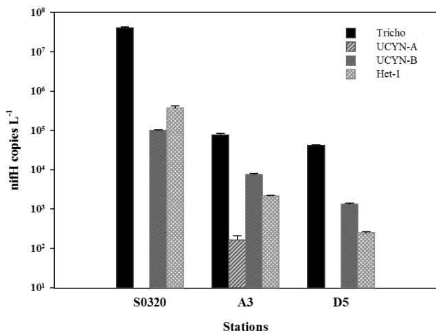
Figure 2. Cyanobacteria diazotroph nifH phylotype abundances ( nifH gene copies L -1 ). Tricho: Trichodesmium spp.; UCYN: unicellular N 2 -fixing cyanobacteria from Group A, B; Het-1: heterocystous cyanobacteria from Group 1. Error bars represent the standard deviation for triplicate natural samples.
