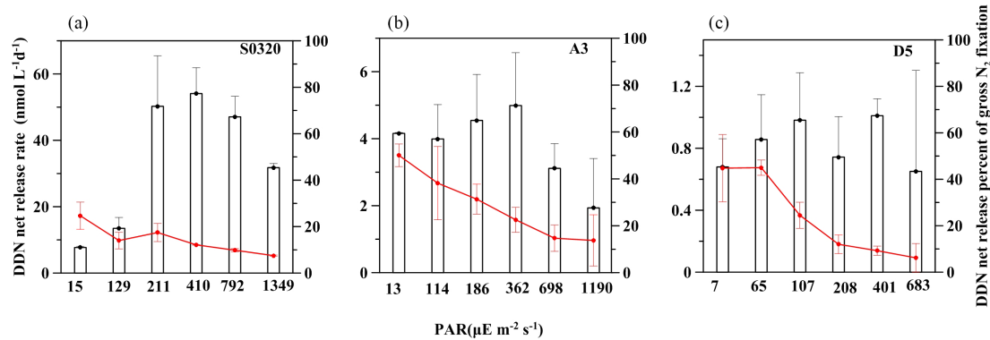
Figure 5. DDN net release rate (bar charters) and percentage of total NF (red lines) under different light intensities for stations S0320, A3 and D5. Error bars represent the standard deviation of triplicates.
