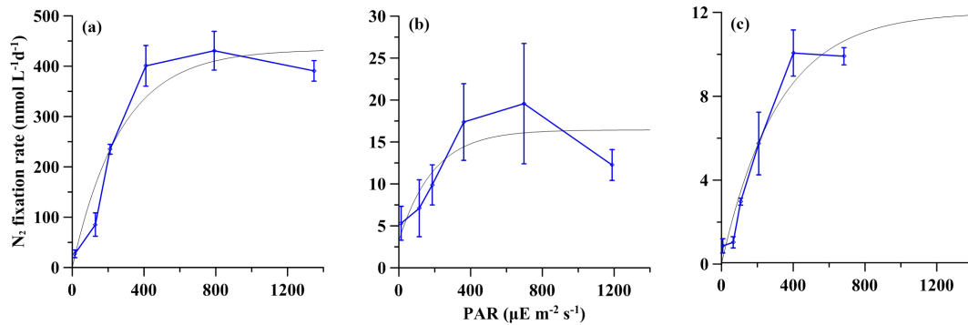
Figure 3. Net (particulate) NF versus irradiance. The gray curves represent the fitted NF-I curves. The error bar represents the standard deviation of triplicate incubations. (a) Station S0320; (b) station A3; (c) station D5.
