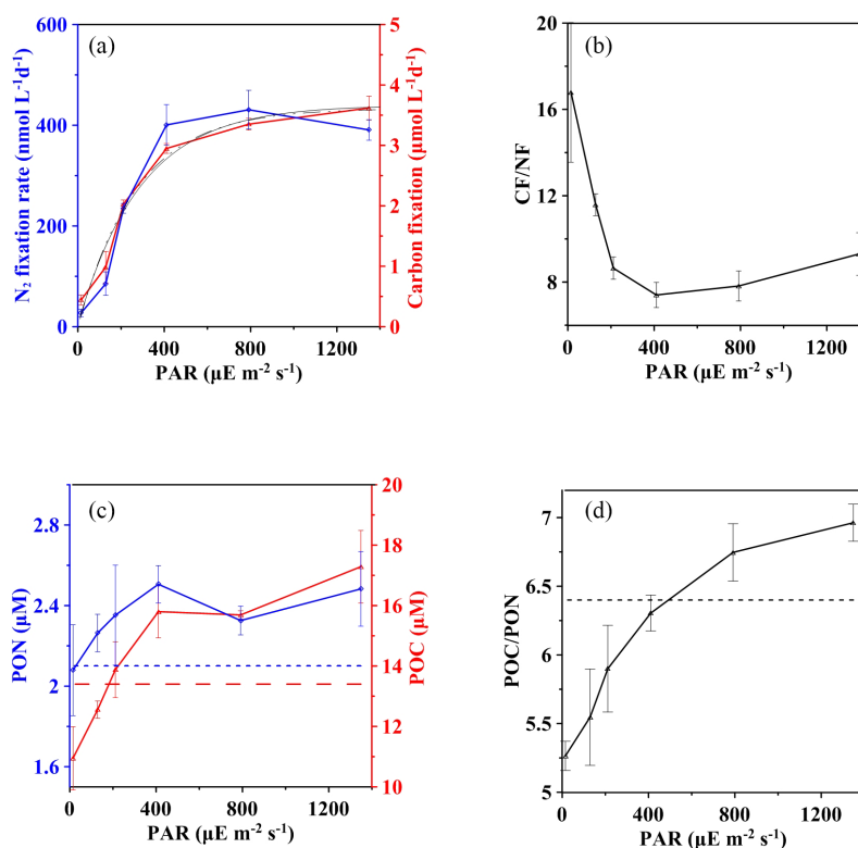
Figure 4. Effect of light on the carbon and nitrogen budget at station S0320 with a Trichodesmium thiebautii bloom. (a) Carbon (red solid line) and nitrogen (blue solid line) fixation at different light intensities with fitted light response curves (black solid line for CF and black dotted line for NF). (b) The CF/NF ratios at different light intensities. (c) The final concentrations of POC (red solid line) and PON (blue solid line) after incubations under different light intensities and initial values of POC (red dashed line) and PON (blue dashed line) concentration. (d) C/N ratios after incubation in different light conditions. Error bars represent the standard deviation of triplicates.
