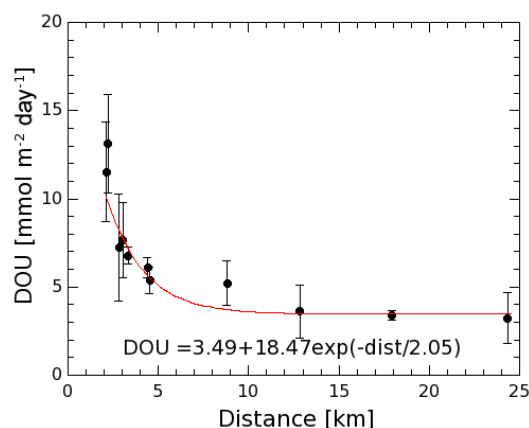
Figure 3. Diffusive oxygen uptake (DOU) across the sediment–water interface as a function of the distance from the Rhône River mouth. The fluxes decrease exponentially following \text{DOU} = F_{\min} + Ae^{(-x/t)} , with F_{\min} being the flux in the offshore region, x the distance to the river mouth in km and A and t being the numerical constants. Error bars are standard deviations between the diffusive fluxes calculated from the five single oxygen profiles measured at each station.
