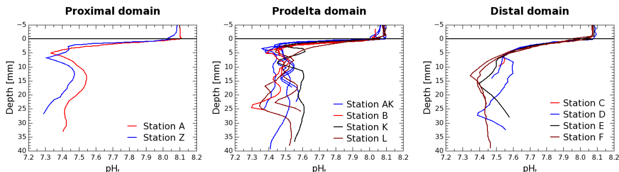
Figure 4. All pH t micro profiles measured during the DICASE cruise in the proximal, the prodelta and the distal domains. The sediment–water interface is marked by a horizontal line.
