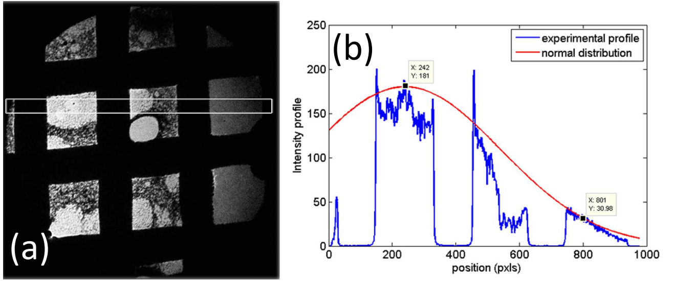
FIG. 3. Measurement of the intensity distribution in the cone angle (a) counting mode imaging of the sample shadow ( V = -360 V, I = 0.012 pA); (b) in blue: intensity profile along the white rectangle in (a) and in red: normal distribution with a standard deviation \sigma = (300 \pm 50) pxls.
