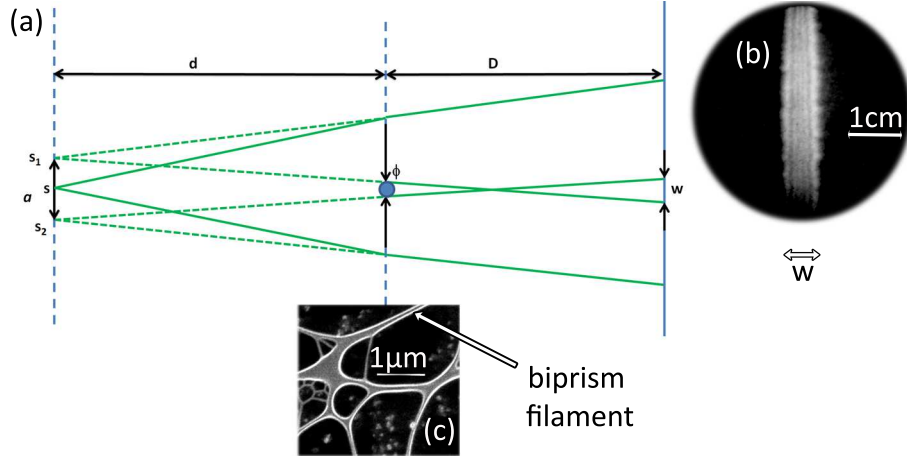
FIG. 5. (a) Geometrical representation of the experiment where s is the real source and \phi , the biprism diameter; s_1 and s_2 are the “virtual sources” (b) Analog recording of the electron projection of the biprism: interference pattern from s_1 and s_2 in the plane of the detector appears in w ; (c) Scanning electron microscope view of the filament used as biprism in the experiment, width about \phi = 118 nm.
