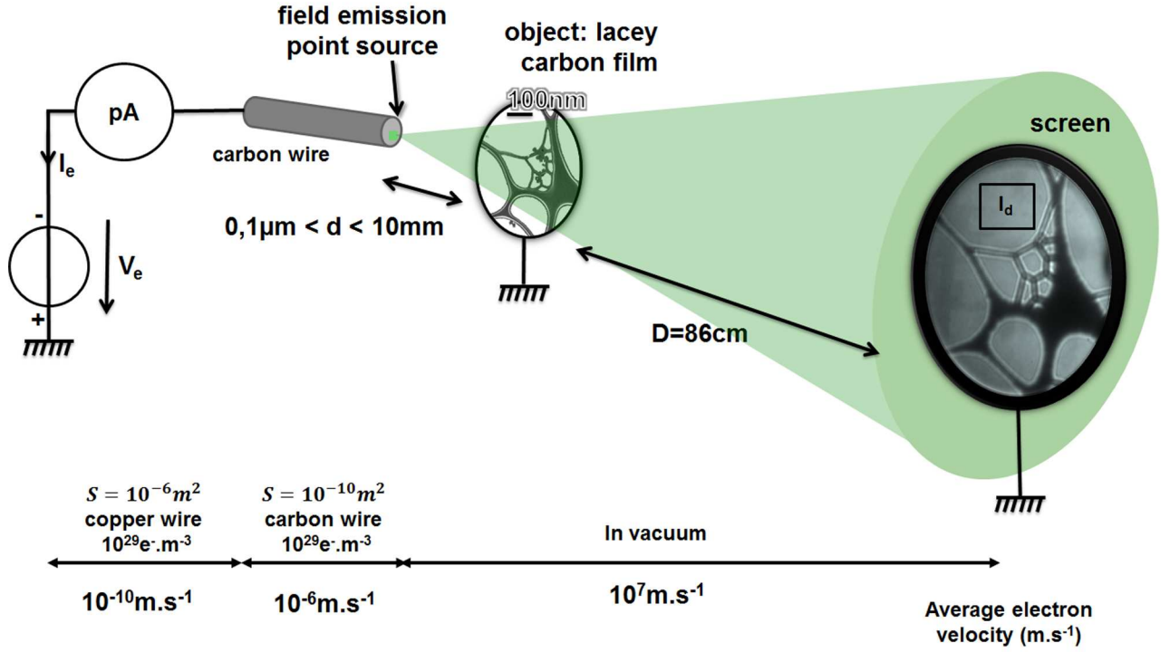
FIG. 1. Low-energy electron microscope. A field emission source, biased to some V_e = -100 V through a picoammeter, illuminates a lacey carbon film. The physical shadow of the film is observed on a dual stage micro-channel plate fluorescent screen assembly. Example of electron velocities are given for V_e = -1000 V and I_e = 1 \mu\text{A} .
