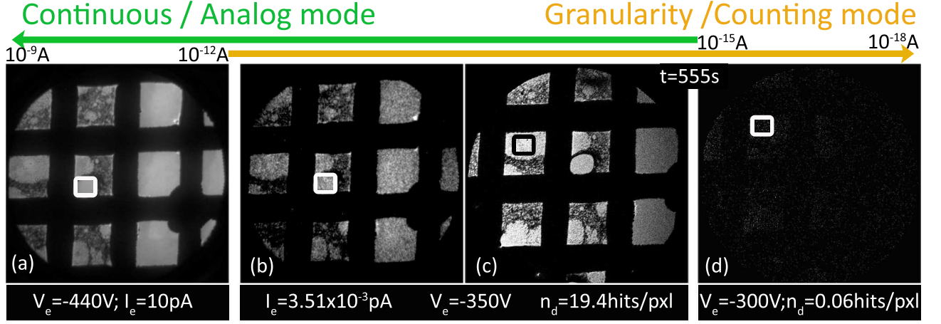
FIG. 2. Depending on electron detection, continuous intensity or granularity of electrons are illustrated (a) For a few picoamps, picoammeter and gray level detection are required; gray level gives the intensity calibration; (b) For a few femtoamps, analog intensity is measured through the gray level when (c) the counting mode gives the number of detected hits; (d) For a few attoamps, the number of detected hits is given for the highest-intensity zone. Measurements are performed in rectangles.
