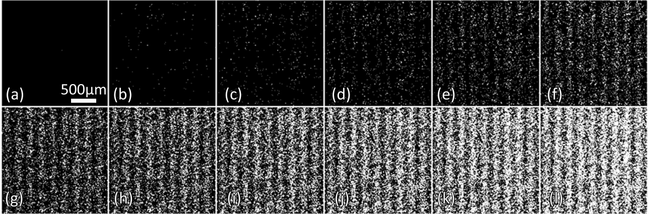
FIG. 6. Interference pattern buildup. Emission voltage V_e = -227 V, source-object distance d = 18 \mu\text{m} , inter-source distance a = 294 nm, object-detector distance D = 86 cm. The fringe distance i = 0.24 mm. (a) t = 10 \times 111 ms; (b) t = 11 \times 10 \times 111 ms; (c) t = 21 \times 10 \times 111 ms; (d) t = 31 \times 10 \times 111 ms; (e) t = 41 \times 10 \times 111 ms; (f) t = 51 \times 10 \times 111 ms; (g) t = 61 \times 10 \times 111 ms; (h) t = 71 \times 10 \times 111 ms; (i) t = 81 \times 10 \times 111 ms; (j) t = 91 \times 10 \times 111 ms; (k) t = 102 \times 10 \times 111 ms; (l) t = 112 \times 10 \times 111 ms.
