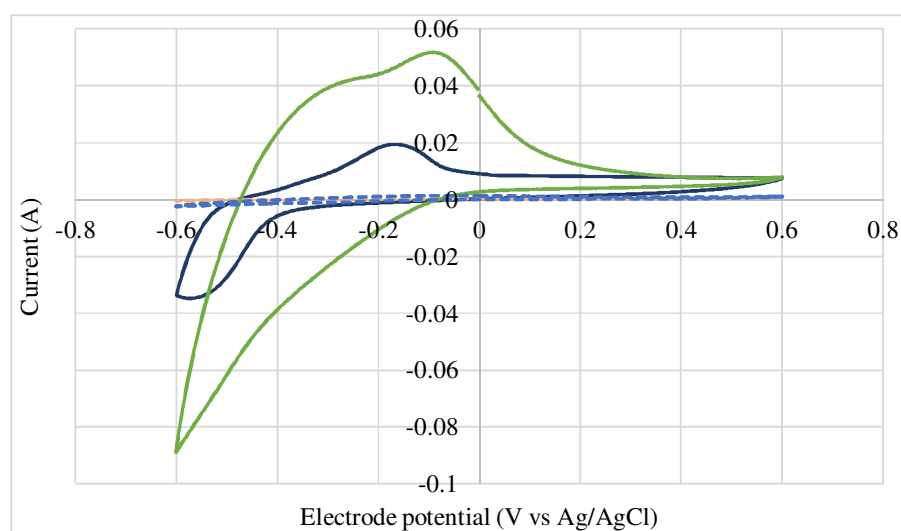
Figure 3: Cyclic Voltammeteries between -0,6V and +0,6V at 20mV/s of Working Electrode at initial time (dot lines) and final time (full line) in BES1 (blue line), BES2 (green line) and abiotic control (orange line).
