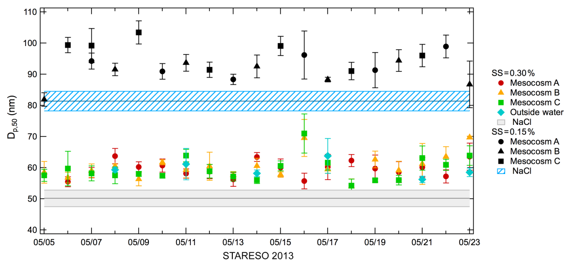
Figure 7. Activation diameters at SS = 0.30 % and SS = 0.15 %. The shaded and striped areas indicate the NaCl activation diameters at each given supersaturation as a direct comparison to the seawater samples.
