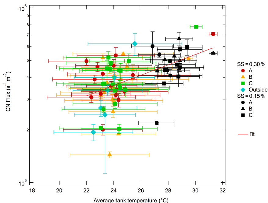
Figure 4. Particle flux calculated for a 9 \text{ m s}^{-1} wind speed versus average tank temperature for both supersaturations tested.
