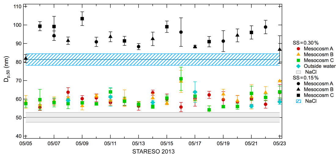
Figure 7. Activation diameters at SS = 0.30 % and SS = 0.15 %. The shaded and striped areas indicate the NaCl activation diameters at each given supersaturation as a direct comparison to the seawater samples.
