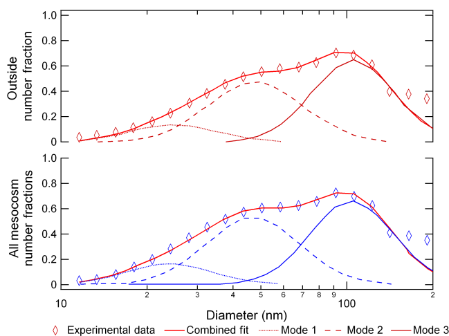
Figure 2. Average size distributions of the outside water and all mesocosms (A, B and C) at both supersaturations (SS = 0.30 and 0.15 %) used in this study. The mesocosms are fit with three different log-normal modes.
