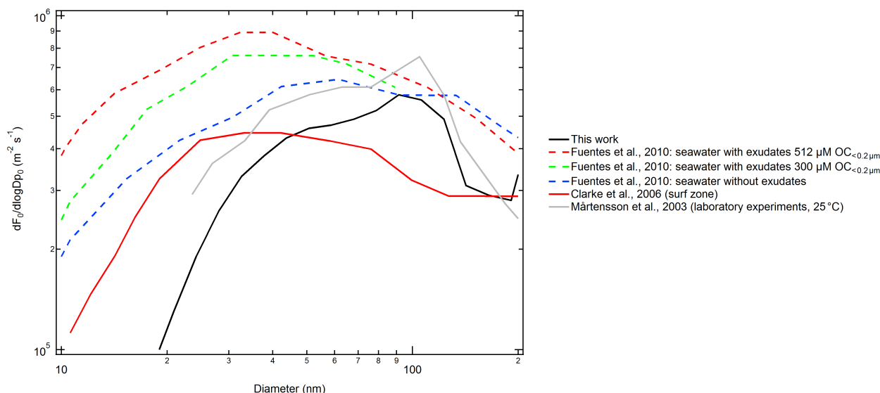
Figure 5. Comparison of size-resolved source flux measurements from previously published work and this work.
