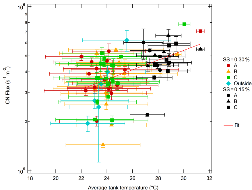
Figure 4. Particle flux calculated for a 9 \text{ m s}^{-1} wind speed versus average tank temperature for both supersaturations tested.
