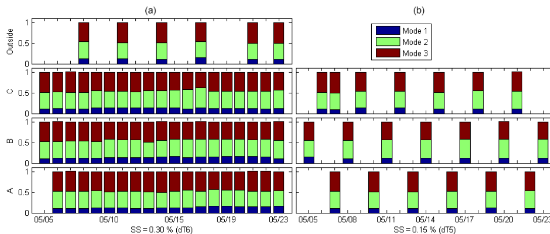
Figure 3. Number fraction of SMPS log normal modes in mesocosms A, B and C and outside water at \text{SS} = 0.30\% (a) and \text{SS} = 0.15\% (b).
