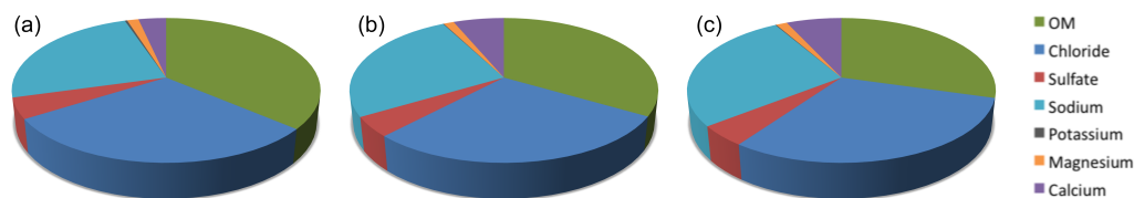
Figure 6. Average chemical composition of the PM 1 PMA generated from seawater of (a) mesocosm A (control), (b) mesocosm B (enriched) and (c) mesocosm C (enriched).
