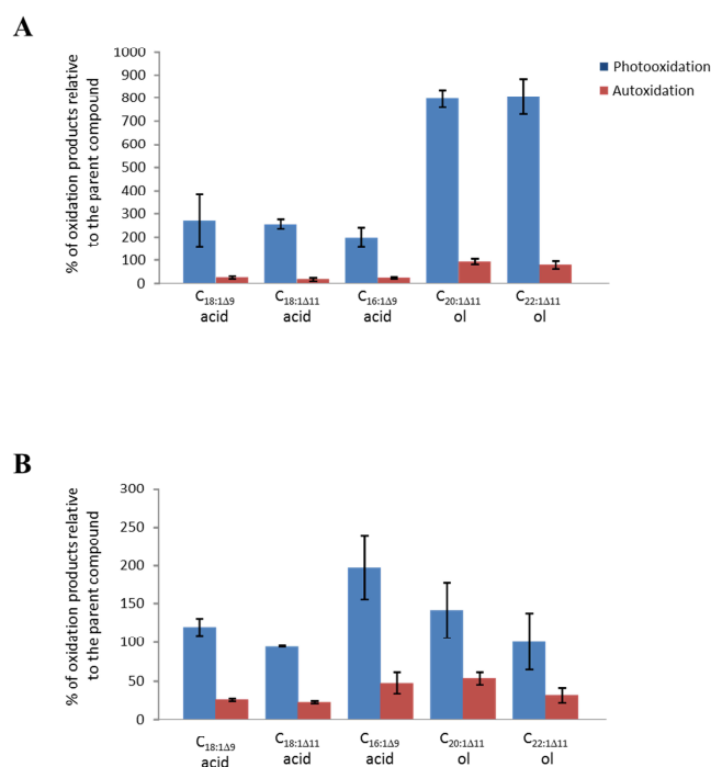
Fig. 3. Percentages of photooxidation and autooxidation products (relative to the residual parent compound) of monounsaturated fatty acids and alkan-1-ols observed in G09-A2 (A) and G09-A3 (B) samples.
