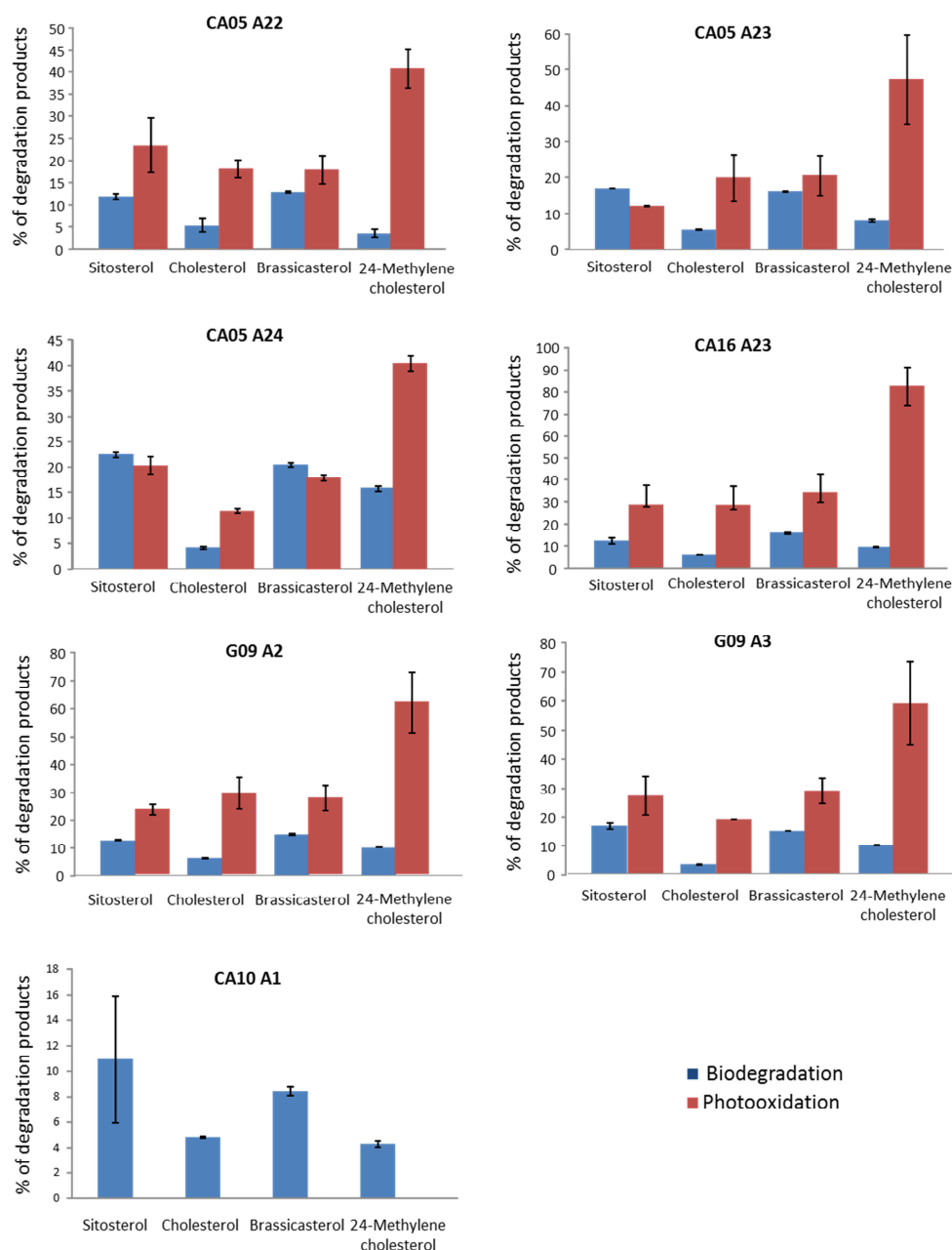
Fig. 8. Percentages of photooxidation and autooxidation products (relative to the residual parent compound) of sitosterol, cholesterol, brassicasterol and 24-methylenecholesterol in the different samples investigated.
