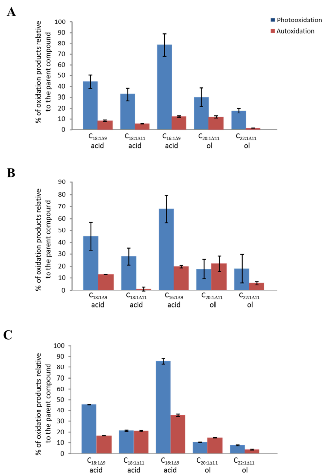
Fig. 4. Percentages of photooxidation and autooxidation products (relative to the residual parent compound) of monounsaturated fatty acids and alkan-1-ols observed in CA05-A22 (A), CA05-A23 (B) and CA05-A24 (C) samples.
