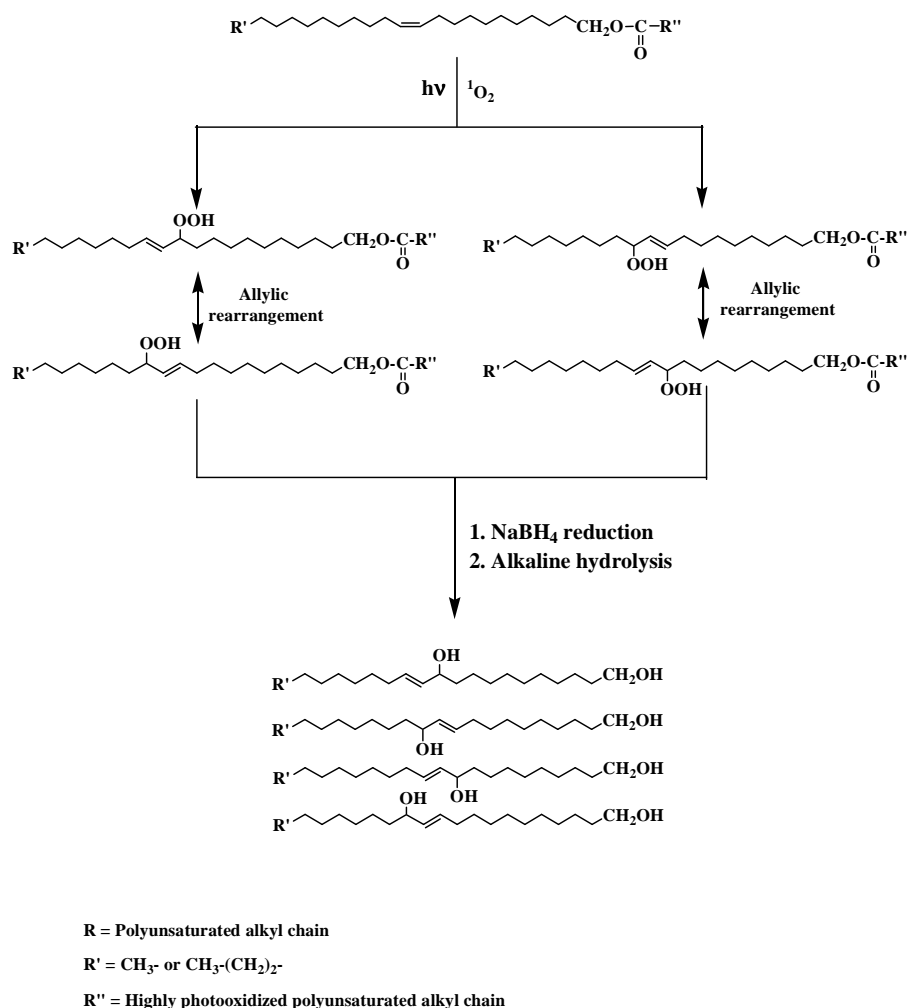
Fig. 6. Type II (i.e. involving singlet oxygen) photooxidation of \text{C}_{20:1\Delta 11} and \text{C}_{22:1\Delta 11} alkan-1-ols.
