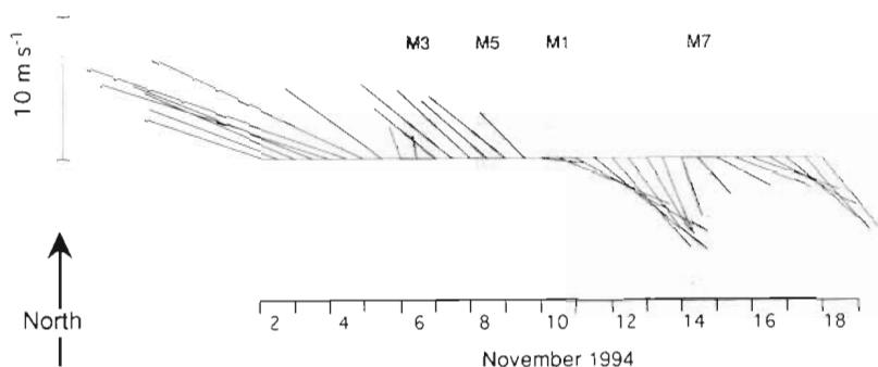
Fig. 2. Stick plot of the wind speed and direction measured near Marseilles between 2 and 18 November 1994. Sticks are rotated by 180^\circ to indicate the leeward direction of the wind. Values are averaged over 12 h periods and are smoothed using 2 repeated passes of a simple hanning window. The days on which the 4 stations were sampled are shown by vertically shaded bars
