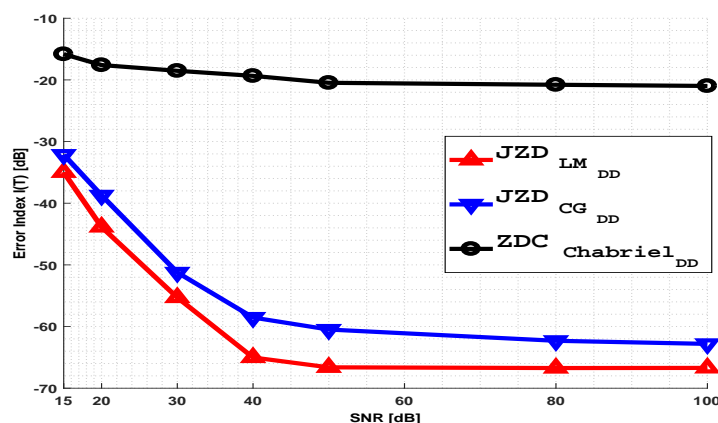
Figure 6. Comparison of the different methods: evolution of the error index I(\mathbf{T}) in dB versus SNR
