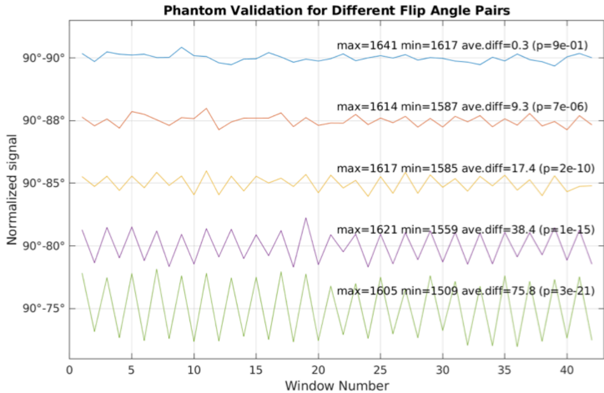
Figure 3: Demonstration of the temporal information extracted using the dynamic ^{23}\text{Na} MRI acquisition ^{23}\text{Na} signal variations obtained on a phantom at \text{TE}_1=0.2\text{ms} and reconstruction on a phantom. Every 30s, acquisition parameters (flip angles) varied leading to a significant ^{23}\text{Na} MR signal change that could be easily be observed.
