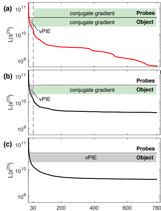
Fig. 6. Evolution of the criterion \mathcal{L}(s^{(n)}) for different reconstruction strategies. For each method, labelled (a) to (c), colored patterns remind which algorithm is used and which variable is updated, either the object only or both object and probes.
