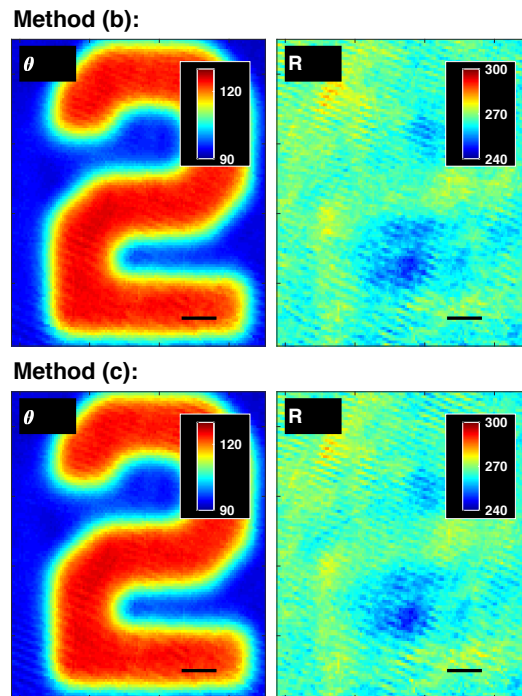
Fig. 5. Retrieved optical properties of the test target, obtained with methods (b) and (c), to be compared with Fig. 4. Scale bar is 25 \mu\text{m} .
