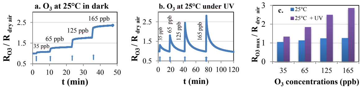
Fig. 3. Sensor responses as function of O_3 concentrations at 25^\circ C (a) in dark, (b) under UV and (c) comparison of both.
