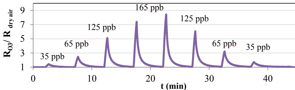
Fig. 4. Ozone exposure during 30s increasing from 35 to 165 ppb and decreasing from 165 to 35 ppb at 125^\circ C under UV.
