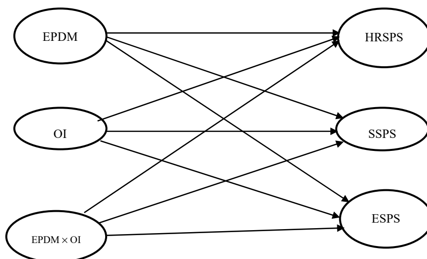
Figure 2. Structure regression model in AMOS for hypotheses testing. Notes: EPDM × OI is the product term of the interaction between these variables. For greater simplicity and clarity, we do not show covariances among independent variables, the item-level structure of the constructs, or error terms of dependent variables.
