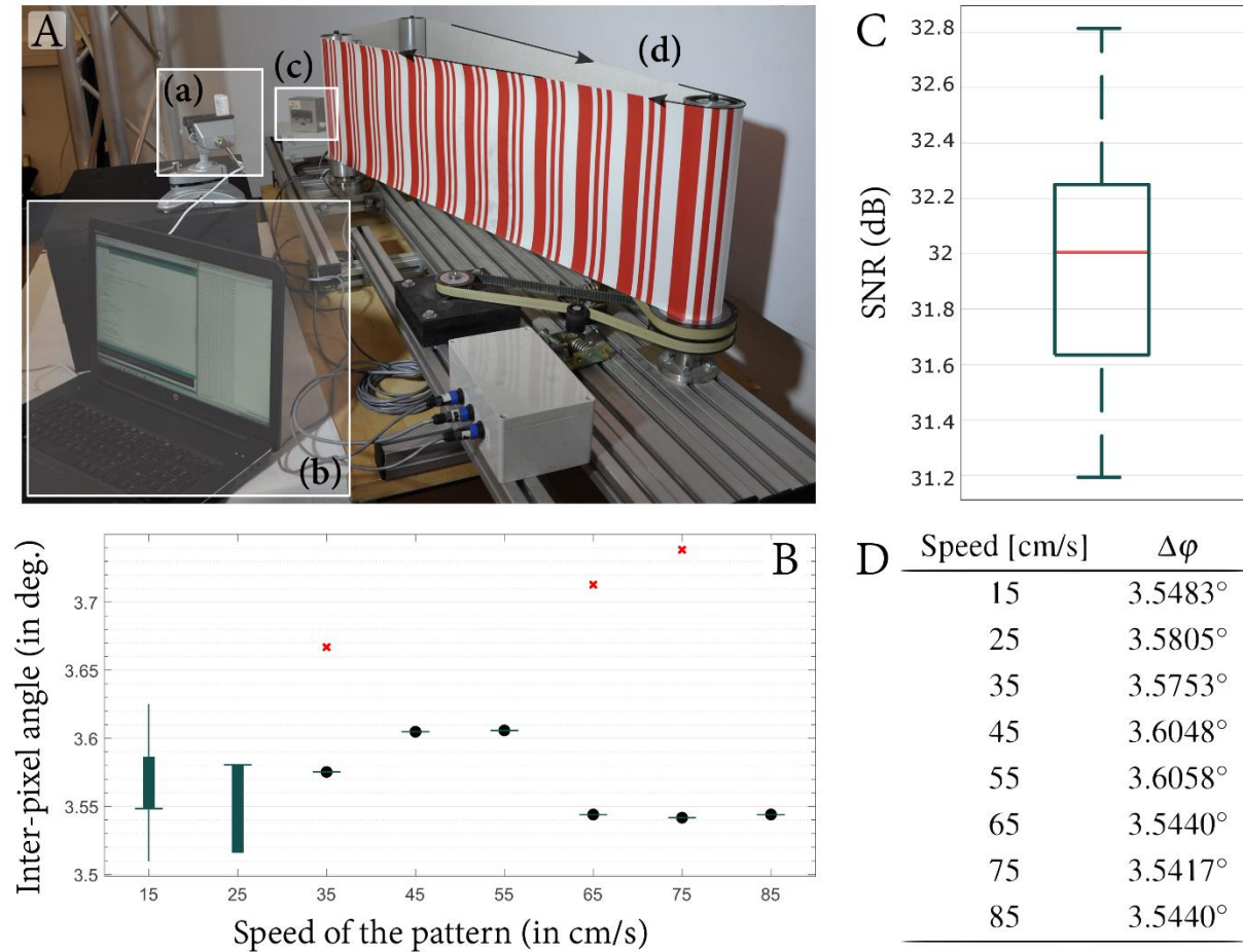
Fig. S8. Characterization of the M²APix optic flow sensor. The benchmark setup is shown in (A) where: (a) is the M²APix sensor oriented toward a moving pattern (d) consisting of parallel red stripes. The speed of the pattern was measured with a tachometer (c). Data were collected on a laptop (b). (B) Boxplot of the inter-pixel angle measured at pattern speeds ranging from 15cm/s to 85cm/s. The mean value based on all the experiments, which was used in the optic flow calculations on-board AntBot was equal to 3.57°, with a low standard deviation (0.027°). (C) Boxplot of the SNR values. (D) Mean values of the inter-pixel angle. The mean signal-to-noise ratio (SNR) value was equal to 31.97dB, with a standard variation of 0.44dB. The SNR was taken to be the inverse of the sensor's coefficient of variation.
