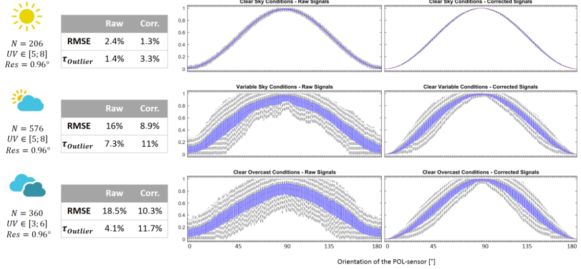
Fig. S6. Characterization of the celestial compass. The UV_0 and UV_1 POL-units' responses within [0, 180^\circ] were collected and normalized. Distributions at each orientation of the polarized filter are shown, and the mean responses are indicated by red lines. The root-mean-square error (RMSE) is given as a percentage of the overall number of points collected. The percentage of outliers detected is also specified. Results are compared between clear (top), variable (middle) and overcast (bottom) sky conditions. Mean UV-indexes are given under clear sky conditions.
