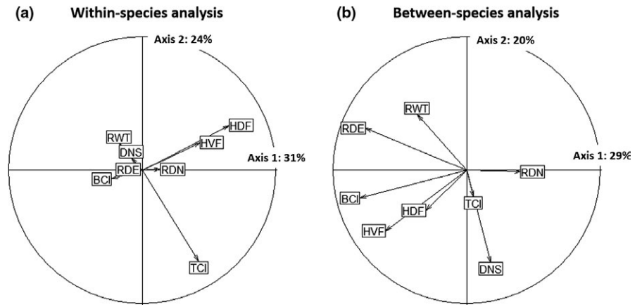
FIGURE 2 Correlation circles regarding the first two axes of the (a) within-species and (b) between-species PCA on functional traits for tadpole communities from Atlantic Forest. BCI: Body compression index; DNS: Distance from nares to snout; HDF: Relative height of the dorsal fin; HVF: Relative height of the ventral fin; RDE: Relative diameter of the eyes; RWT: Relative width of the tail; RDN: Relative diameter of the nares; TCI: Tail compression index
