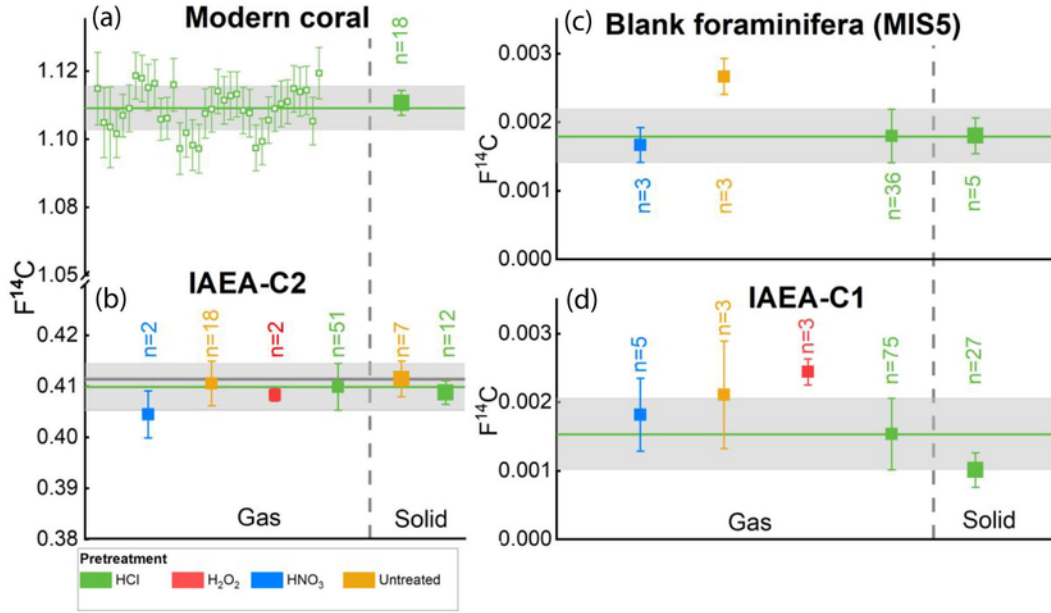
Fig. 1. F^{14}C values of gas and solid measurements of standard and blank samples with standard size (residual mass after leaching of \approx 100 \mu\text{gC} and \approx 500\text{--}1000 \mu\text{gC} for gas and solid measurements respectively). (a) Modern coral ( Porites from Moorea, Aix-13027), (b) IAEA-C2 reference material, (c) foraminiferal samples picked from a > 100 kyr sediment layer (marine isotopic stage 5 from a sediment core raised off Morocco) and (d) IAEA-C1 reference material. Data summarized in this figure were measured over a period of two years. The colors stand for the different pretreatments applied before the final hydrolysis with \text{H}_3\text{PO}_4 (HCl is used routinely, while \text{HNO}_3 and \text{H}_2\text{O}_2 have also been tested). Empty green symbols show individual gas measurements pretreated with HCl, while solid symbols represent the arithmetic mean with the associated standard deviation for both gas (left) and solid (right) measurements. The horizontal light grey bar indicates the arithmetic mean and associated standard deviation of gas samples leached with HCl, while the darker grey bar (panel b) indicates the consensus value and associated error for the reference material IAEA-C2. The results for the modern coral and IAEA-C2 were corrected for a blank value based on IAEA-C1 samples measured in the same magazine. By contrast, the results for IAEA-C1 and blank foraminifera are reported as raw F^{14}C without background correction. (For interpretation of the references to colour in this figure legend, the reader is referred to the web version of this article.)
