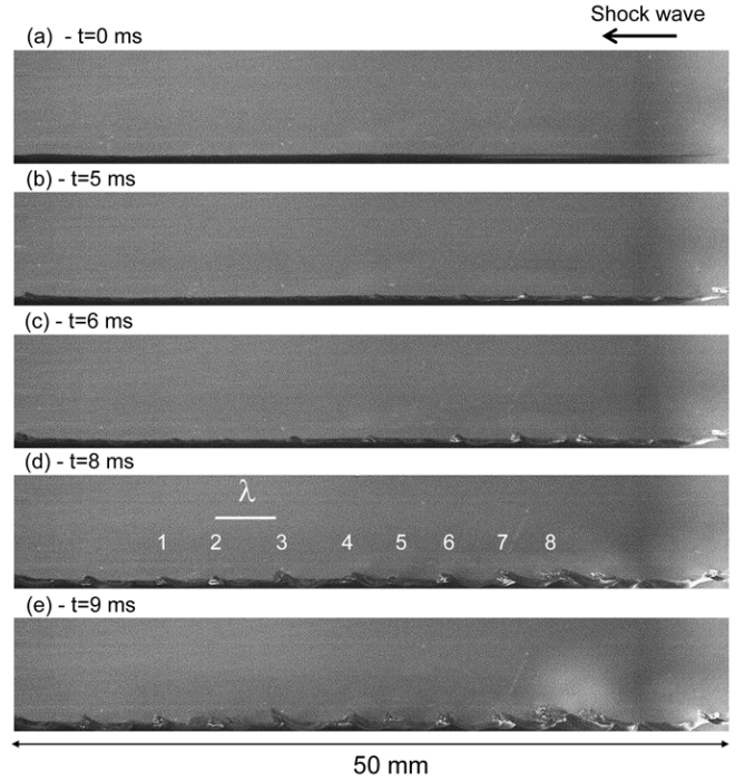
Fig. 1 Sequence of pictures showing the interaction of an incident shock wave of Mach number M_{is}=1.11 with a layer of water 10 mm deep. \lambda represents the distance between each rolls numbered from 1 to 8.
