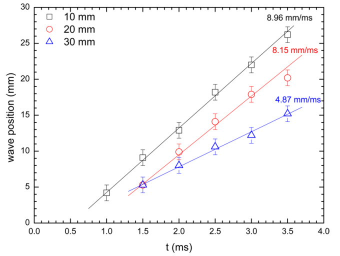
Fig. 6 Motion of traveling wave induced by shocked air flow for three depths of water. The incident shock-wave Mach number M_{is}=1.43 .
