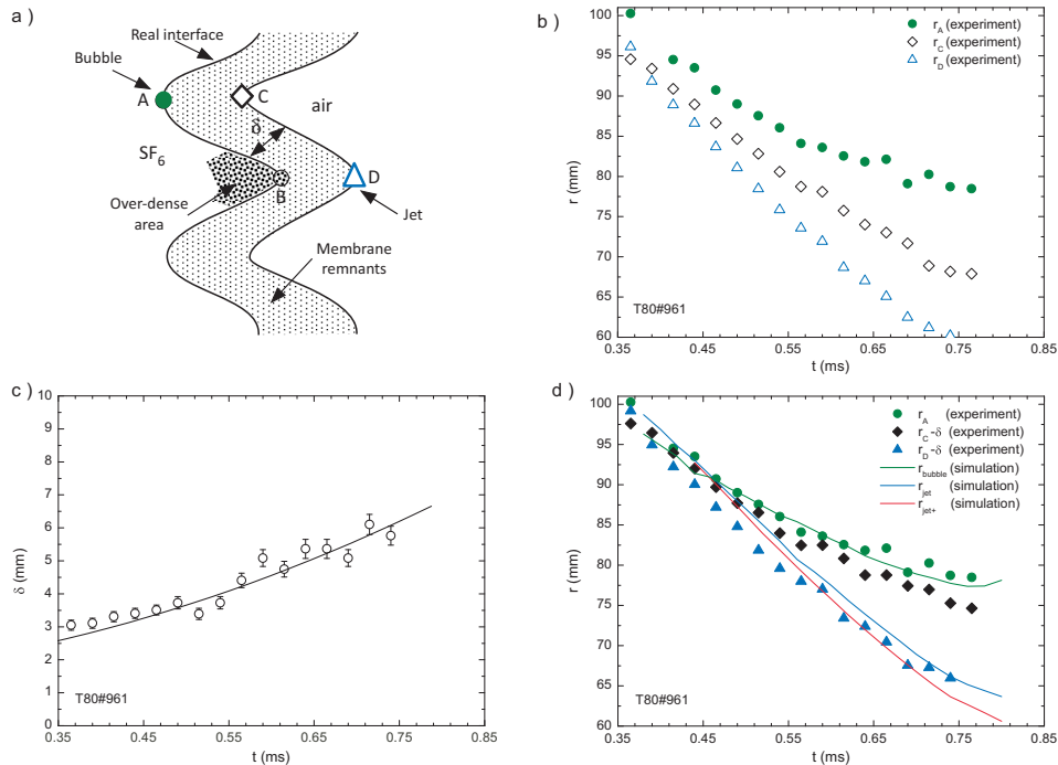
FIG. 14: Interface study for the shot #961. a- Schematic of the Schlieren picture, b- experimental location for points A, C, D , c- growth of the foamy zone, d- comparison between numerical and experimental estimates of the locations of the interface peak and valley. Symbols are obtained from the experiments and formula (4). Curves are from the numerical simulations. For the trajectory of the jet, the two curves are obtained by taking into account or not the extra small jet which is induced by the grid.
