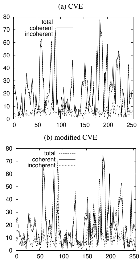
FIG. 2: One dimensional cuts in the x -direction, for y = z = 32\Delta x with \Delta x = \frac{2\pi}{256} for the modulus of vorticity |\bar{\omega}| for total field, coherent and incoherent fields at R_\lambda = 140 .
