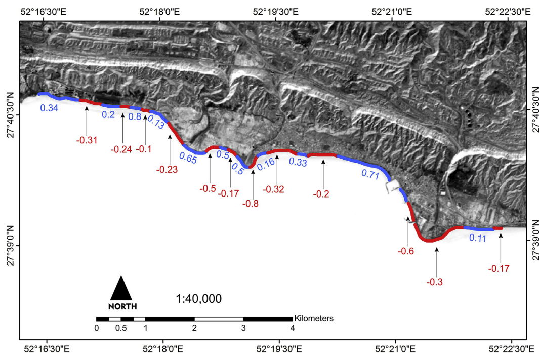
Fig. 4. Map of average EPR erosion/accretion rates, in \text{m yr}^{-1} , for the period 1973–2016.
