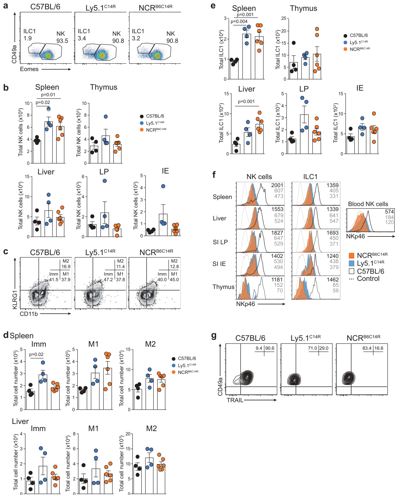
Figure 6. Loss of Nkp46 surface expression depends on the C14R mutation in the Ncr1 gene. (A) Dot plots showing the frequency of ILC1 and NK cells in the spleen. Data show representative plots gated on live NK1.1 + lymphocytes excluding T and B cells. (B) Total number of NK cells in spleen, thymus, liver, small intestine lamina propria (LP) and within the intestinal intraepithelial compartment (IE). Data are pooled from two independent experiments and show the mean \pm SEM ( n = 4-6 mice/genotype). P values were calculated using an unpaired two-tailed Student's t test. (C) FACS plots showing the frequency of immature (Imm, KLRG1 + CD11b + ), mature 1 (M1, KLRG1 + CD11b + ) and mature 2 (M2, KLRG1 + CD11b + ) NK cells in splenic NK1.1 + CD3 + CD19 + NK cells. (D) Total number of Imm, M1 and M2 NK cells in the spleen and liver of C57BL/6, Ly5.1 C14R and NCR B6C14R mice showing the mean \pm SEM pooled from two experiments ( n = 4-6 mice/genotype). P values were calculated using an unpaired two-tailed Student's t test. (E) Total number of ILC1s in spleen, thymus, liver, small intestine lamina propria (LP) and within the intestinal intraepithelial compartment (IE). Data show the mean \pm SEM pooled from two independent experiments ( n = 4-6 mice/genotype). P values were calculated using an unpaired two-tailed Student's t test. (F) Histograms showing the mean fluorescence intensity of Nkp46 in various tissues for NK cells and ILC1 for wild-type (black solid line), Ly5.1 C14R (solid blue) and NCR B6C14R (solid orange). CD3 + cells were used as a control for Nkp46 expression (black dashed line). Data are representative of tissues analyzed in (A-E). (G) Expression of TRAIL on NK1.1 + CD49a + CD3 + CD19 + hepatic ILC1 in C57BL/6, Ly5.1 C14R and NCR B6C14R . Data show representative plots from two independent experiments and indicate the frequency of expression ( n = 4-6 mice/genotype).
