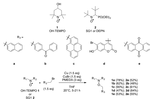
Scheme 1. Synthesis of photosensitive alkoxyamines.
