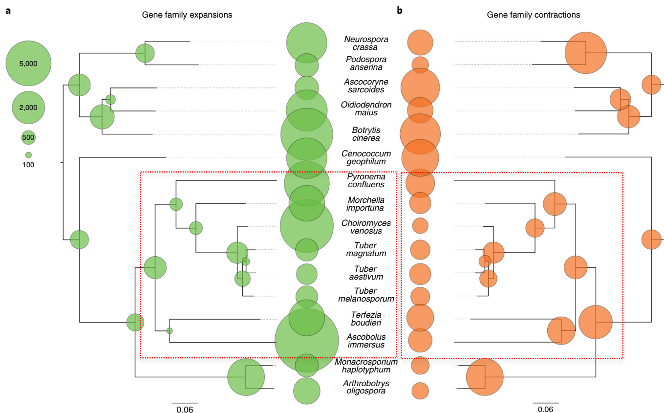
Fig. 2 | Reconstructed gene duplication/loss histories along a time-calibrated phylogeny of 16 fungal species of Ascomycetes. a, b The expansion (green; a ) and contraction (orange; b ) of protein-coding gene repertoires in Tuberaceae and other Pezizomycetes (red box). The analysis was performed using the COMPARE pipeline 27 . The size of the bubbles corresponds to the ancestral number of genes inferred in that node. The scale bar units correspond to gene counts.
