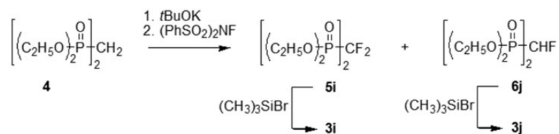
Scheme 2. Synthesis of the mono- and difluorobisphosphonic acids 3i, j.
