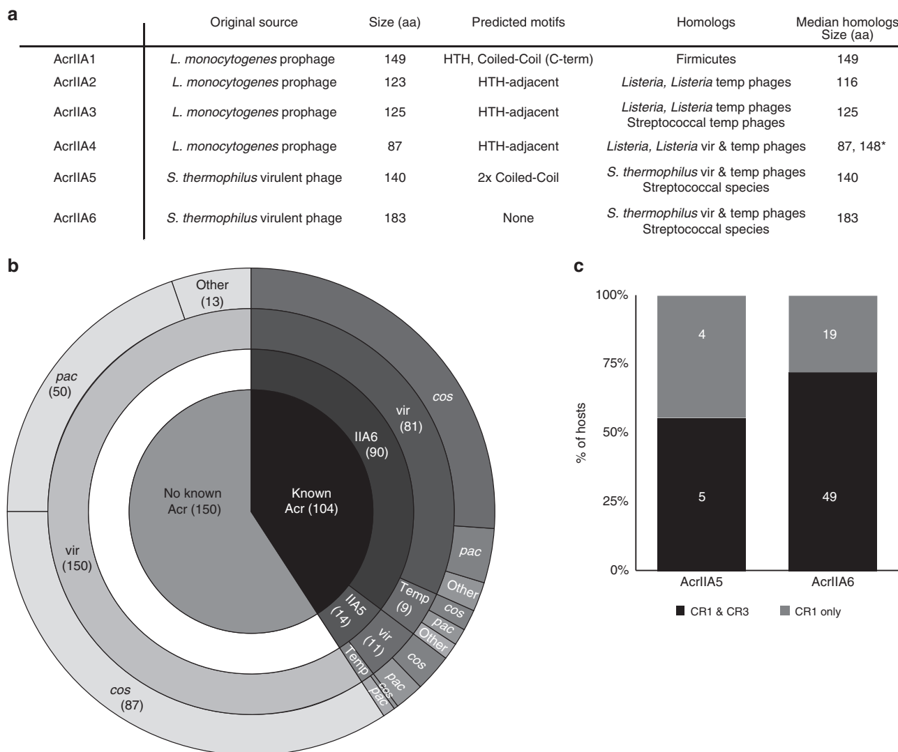
Fig. 2 Bioinformatic analyses of type II-A Acrs. a A summary of key features of type II-A Acrs. For orthologs, virulent and temperate are abbreviated “vir” and “temp,” respectively. The star (*) indicates a bi-modal distribution in size, with a smaller set clustering around 87 aa and a larger set (present in virulent phages) clustering around 148 aa. b Categorizing 254 available S. thermophilus phage genomes for presence of a known Acr, by Acr family, phage type (vir = virulent, temp = temperate), and group (cos, pac, other). c A breakdown of AcrIIA5-containing and AcrIIA6-containing phages by CRISPR-Cas systems present in the host, where the host’s CRISPR types are known. The number of hosts for each category is presented in white over the bar graphs, and no host possesses only the CR3 system
