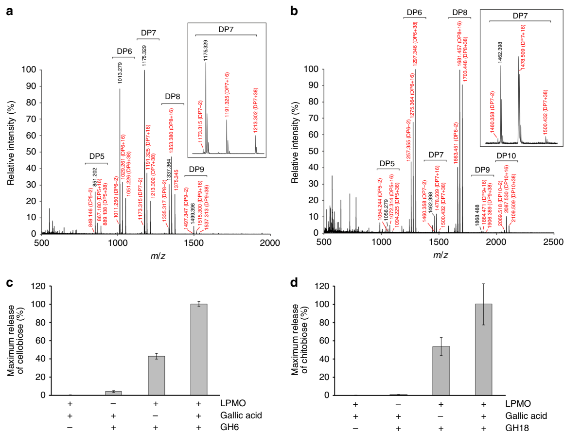
Fig. 3 Biochemical characterization of TdAA15A . MALDI-TOF MS spectrum of products obtained after incubation of 4 mg mL -1 microcrystalline cellulose ( a ) or \beta -chitin ( b ) with 2 \mu M TdAA15A and 4 mM gallic acid for 24 h, showing native and oxidized oligosaccharides. For both substrates, the main peaks correspond to mono- or di-sodiated adducts of C1-alonic acids, imparting +16 or +38 m/z respectively, relative to the mono-sodiated unoxidized form. Smaller peaks for the mono-sodiated lactone (-2) were also identified. All oxidized species are marked in red. For chitin, the products released seem to be predominantly even-numbered oligosaccharides, implying that the enzyme can attack the crystalline structure, as previously observed for other LPMOs 2 . In a and b , 100% relative intensity represents 0.9 \times 10^4 and 1.0 \times 10^4 arbitrary units (a.u.), respectively. Negative control reactions carried out with substrate only, substrate plus gallic acid, and substrate plus TdAA15A did not generate any oxidized products (see Supplementary Fig. 6a–d). Insets are expanded mass spectra for DP7 products. c Relative product quantification, showing release of cellobiose from microcrystalline cellulose by a commercial GH6. The LPMO significantly boosts the activity of the GH6, and such effect is increased by addition of 1 mM gallic acid. d Relative product quantification, showing release of chitobiose from \beta -chitin by a commercial chitinase. The LPMO boosts the activity of the chitinase, and the synergy is further enhanced by the presence of 1 mM gallic acid. All boosting experiments were carried out over 3 h at 28 °C and products quantified by HPAEC. Bars indicate means (error bars: standard deviations of three replicates). The identity and quantity of each species was determined by analysis of commercial standards. See Methods for more details
