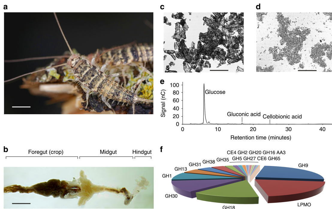
Fig. 1 Discovery of the AA15 LPMO family in T. domestica . (a) Photograph of live specimens of T. domestica in their natural environment. Scale bar, 300 µm. (b) Dissected gut of T. domestica . The crop represents the largest portion of the foregut and the organ where food particles and digestive enzymes accumulate. Scale bar, 100 µm. (c) Microscopic image of Avicel (microcrystalline cellulose). Average particle size is ~50 µm. Scale bar, 30 µm. (d) Microscopic image of food pellet collected from the crop of T. domestica fed on Avicel. Particle size is greatly reduced to ~5 µm. Scale bar, 30 µm. (e) HPAEC analysis of soluble extract isolated from the crop of T. domestica grown on Avicel. One dominant peak corresponding to glucose is clearly visible, plus minor peaks for gluconic acid and cellobionic acid. The identity of the peaks was determined by analyzing commercial standards. (f) Pie chart summary of the CAZymes identified in the crop of T. domestica grown on Avicel. Abundance values for the various families were calculated as molar percentage from emPAI values obtained from shotgun proteomics data (GH9 24.6%, LPMO 20.2%, GH18 13.2%, GH30 12.3%, GH1 8.4%, GH13 4.7%, GH31 4.0%, GH38 3.6%, GH35 2.1%, CE4 1.3%, GH2 1.1%, GH20 1.0%, GH16 0.8%, AA3 0.7%, GH5 0.7%, GH27 0.6%, CE6 0.4%, GH65 0.3%). See Methods for more details
