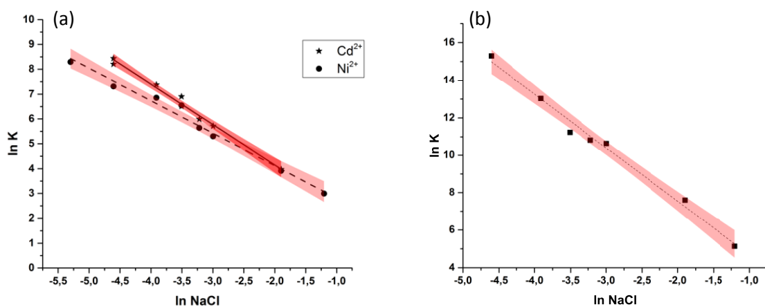
Figure 6: Dependence of the affinity constant on sodium chloride concentration. (a) Dashed and solid lines represent the linear fitting for Cd 2+ and Ni 2+ . (b) Dashed and solid lines represent the linear fitting for Al 3+ . The shade bands around the linear fits represent the confidence interval of 95%.
