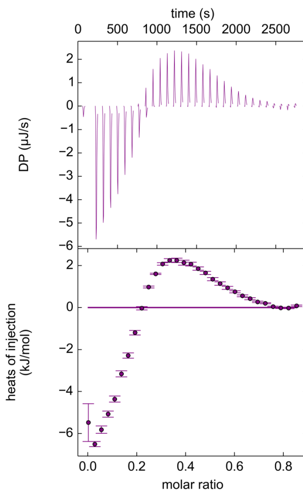
Figure 7: Isothermal titration curve of \text{Cd}^{2+} binding to DNA at 37^\circ\text{C} in TRIS buffer at 5 \text{ mmol.L}^{-1} with NaCl concentration lower than 5 \text{ mM} . The upper curve shows the heat flow versus the time and the lower part shows the heat versus the \text{Cd}^{2+}/\text{DNA-P} molar ratio [41].
