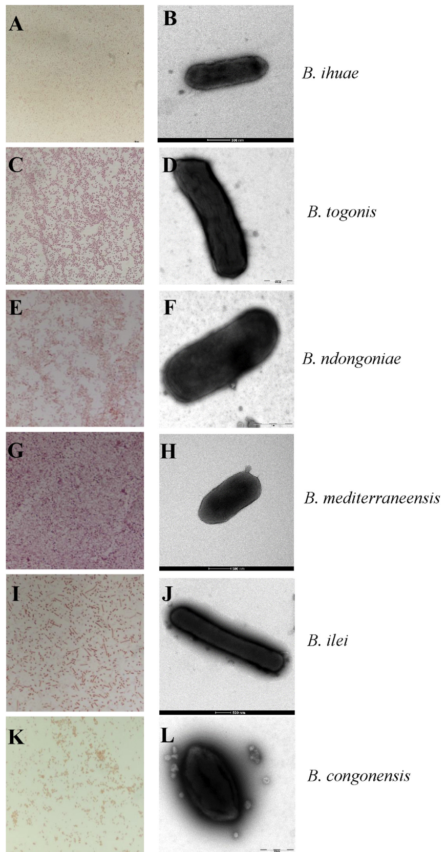
FIG. 4. Gram staining and electron micrographs of Bacteroides new species: B. ihuae (A, B), B. togonis (C, D), B. ndongoniae (E, F), B. mediterraneensis (G, H), B. ilei (I, J) and B. congongensis (K, L), respectively.
