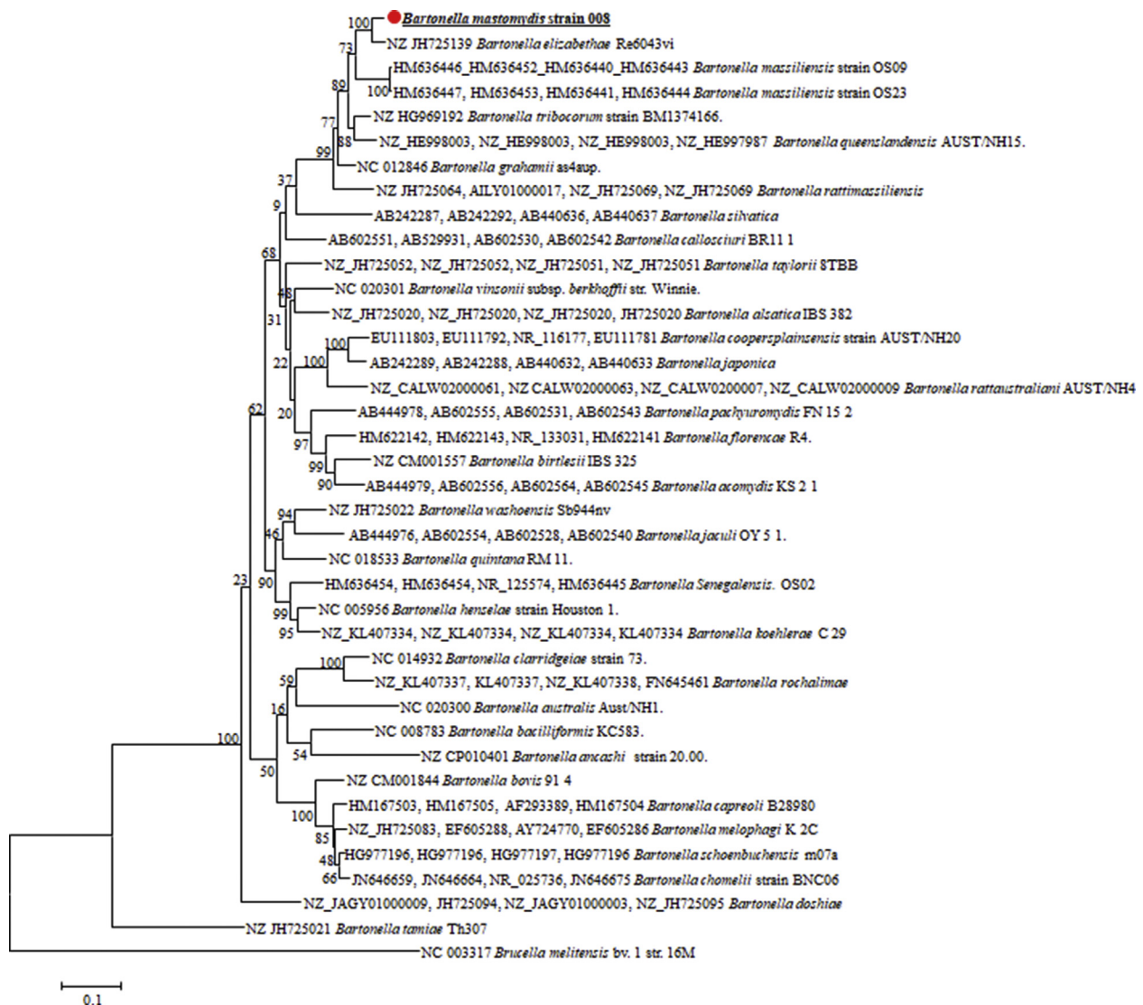
FIG. 1. Evolutionary history of sequenced samples was inferred using maximum likelihood method implemented in MEGA7 [40] and based on concatenated gltA , rpoB , 16S rRNA and ftsZ (total length of 2731 bp) sequences. Sequences of gltA , rpoB , 16S rRNA and ftsZ genes used for comparison were obtained from the GenBank database ( https://www.ncbi.nlm.nih.gov/genbank/ ). Sequences were aligned using BioEdit [41]. Firstly, for each gene individually, sequences we used for comparison were first aligned using CLUSTALWV. All positions containing gaps and missing data were eliminated manually; then each alignment was concatenated and second alignment was performed. Evolutionary history was inferred by maximum likelihood method based on Hasegawa-Kishino-Yano model. Percentage of trees in which associated taxa clustered together is shown next to branches. Initial tree for heuristic search was obtained automatically by applying the Neighbor Joining and BioNJ algorithms to matrix of pairwise distances estimated using maximum composite likelihood (MCL) approach and then selecting topology with superior log likelihood value. Discrete gamma distribution was used to model evolutionary rate differences among sites (two categories (+G, parameter = 0.2144)). Tree is drawn to scale, with branch lengths measured in number of substitutions per site. Statistical support for internal branches of trees was evaluated by bootstrapping with 1000 iterations. Analysis involved 39 nucleotide sequences.
