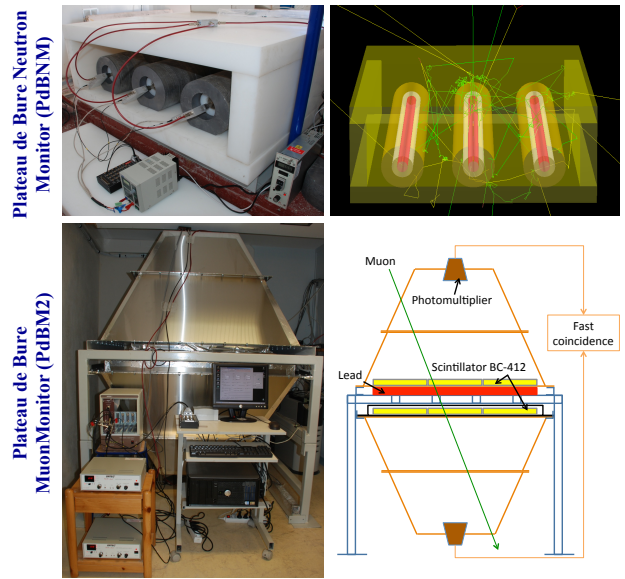
Figure 3. General views (left) and schematics (right) of the Plateau de Bure Neutron monitor (PdBNM) and muon monitor (PdBM2) installed on ASTEP.
