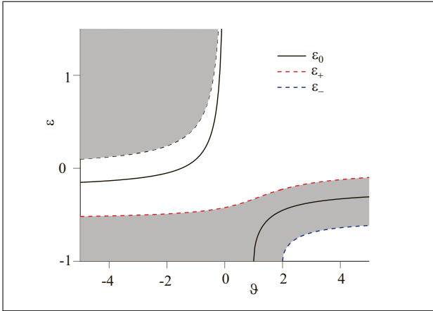
Figure 4. (Colour online) Sketch of the hyperbolicity domains (white) of Murnaghan's law (12) with respect to the parameter \vartheta = (\lambda + 2m)/(\lambda + 2\mu) .
