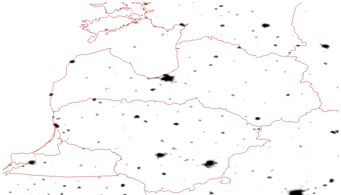
Figure 3: Example of DMSP OLS image from 2000
