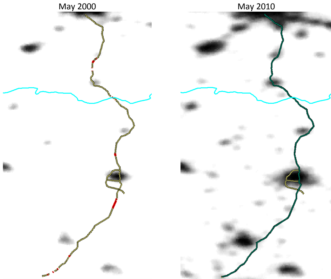
Figure 31: Regional growth of urbanization within the Via Baltica
