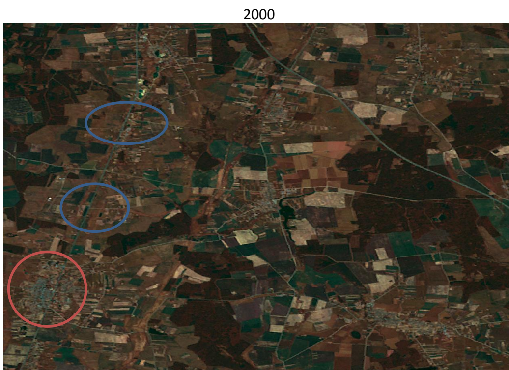
Figure 22: Urbanization of Panevezys Region within the Via Baltica
