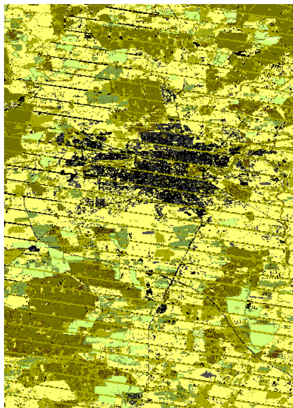
Figure 20 : Example of Panevezys (01/07/2011)
