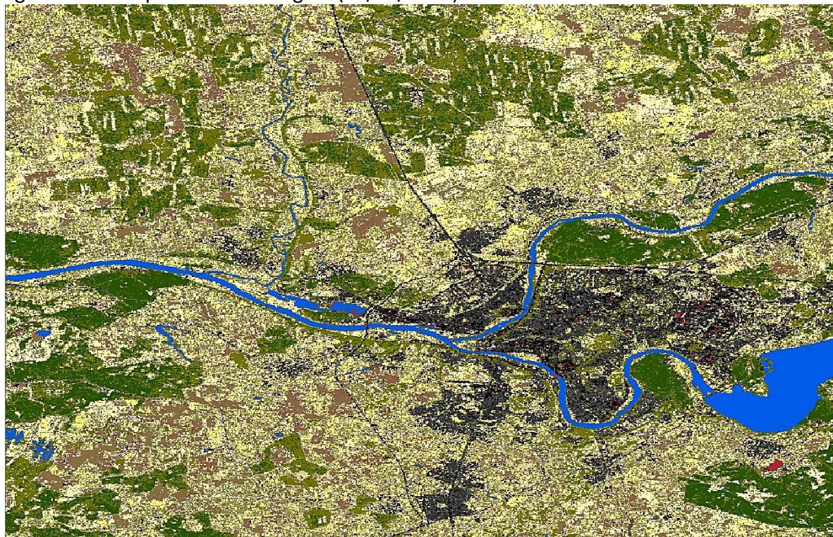
Figure 18: Example of Kaunas region (03/05/2001)
