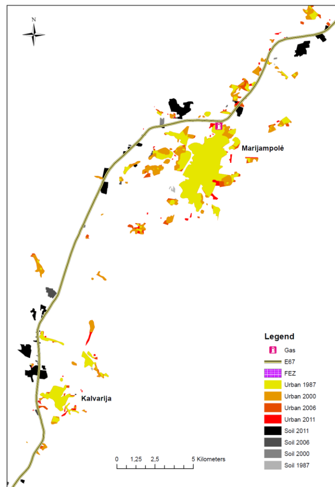
Figure 33: Urban growth of Marijampole and Kalvarija (1987-2000-2006-2011)
