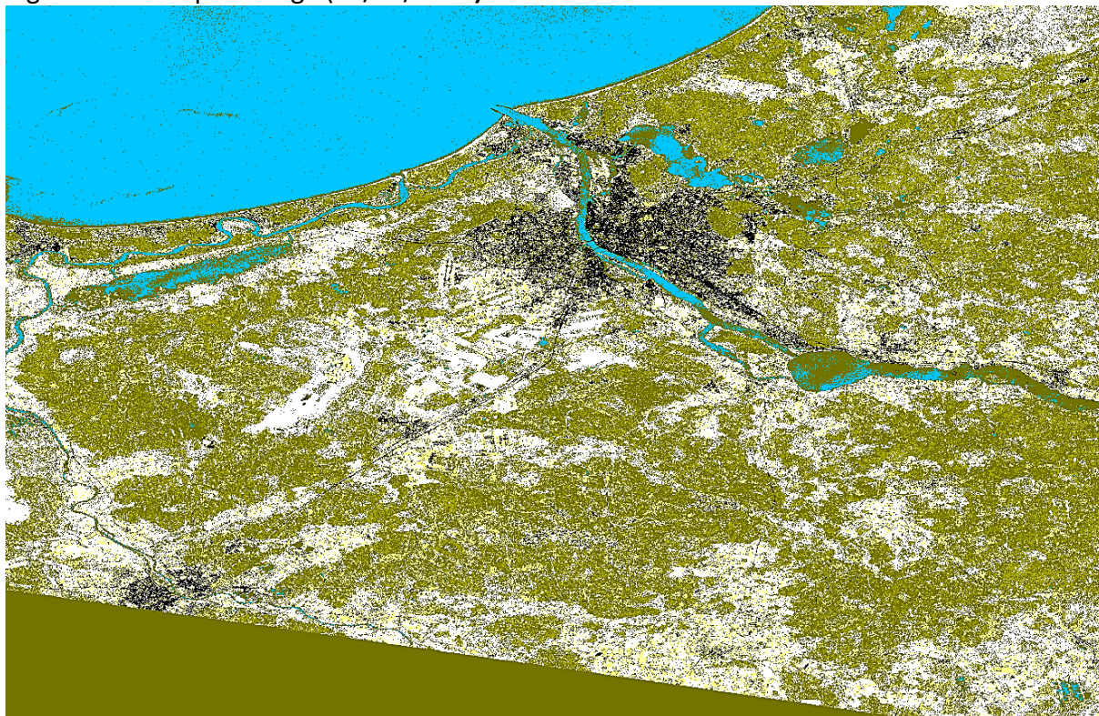
Figure 17: Example of Riga (02/08/1999)
