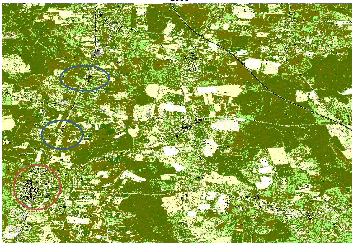
Figure 23: Urbanization of Panevezys Region within the Via Baltica (land cover classification)
