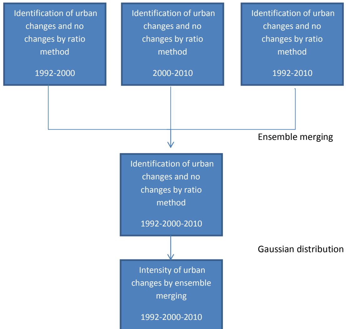
Figure 10: Methodology of urban intensity change modeling
