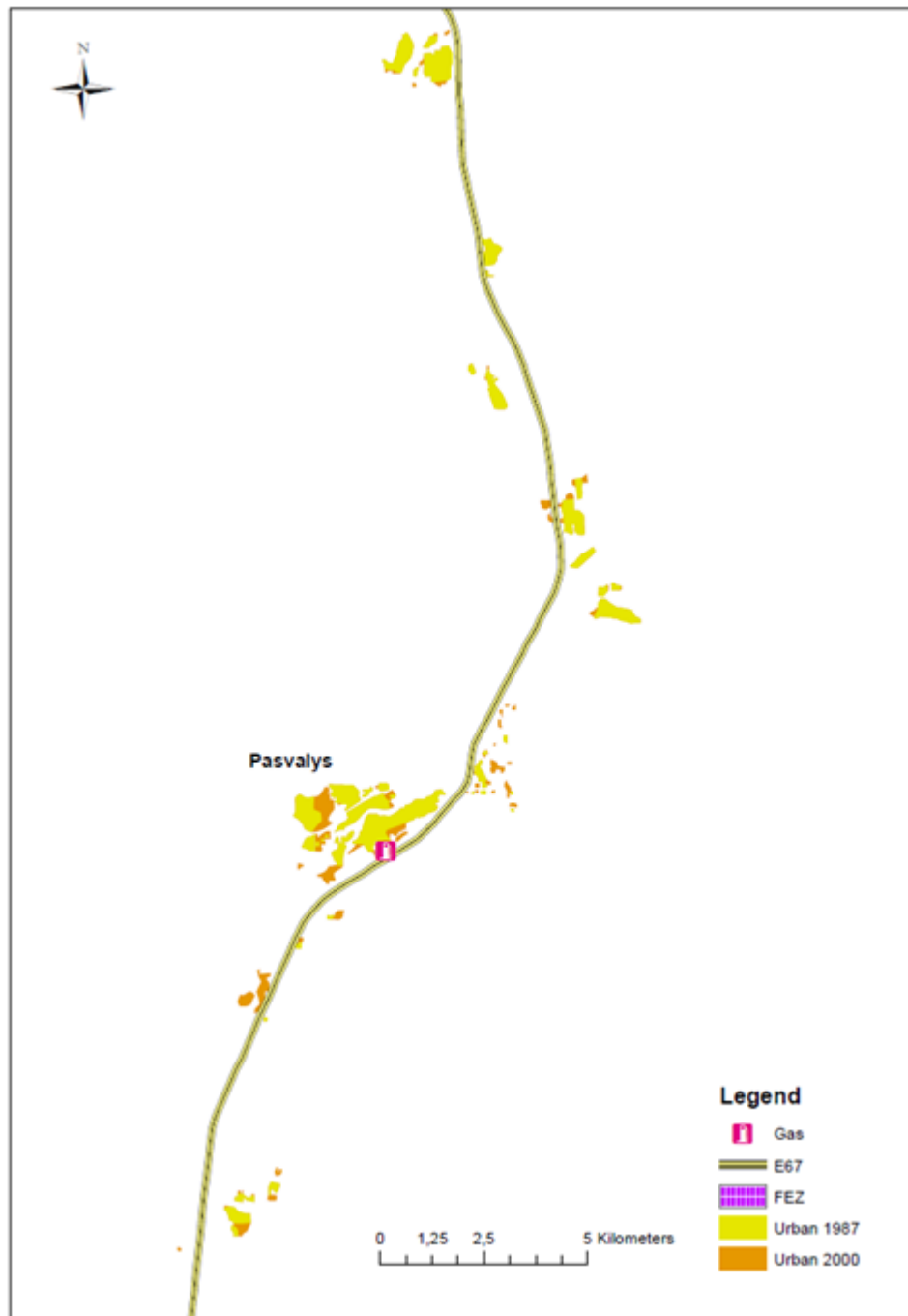
Figure 26: Urban evolution of Pasvalys region (1987-2000)
