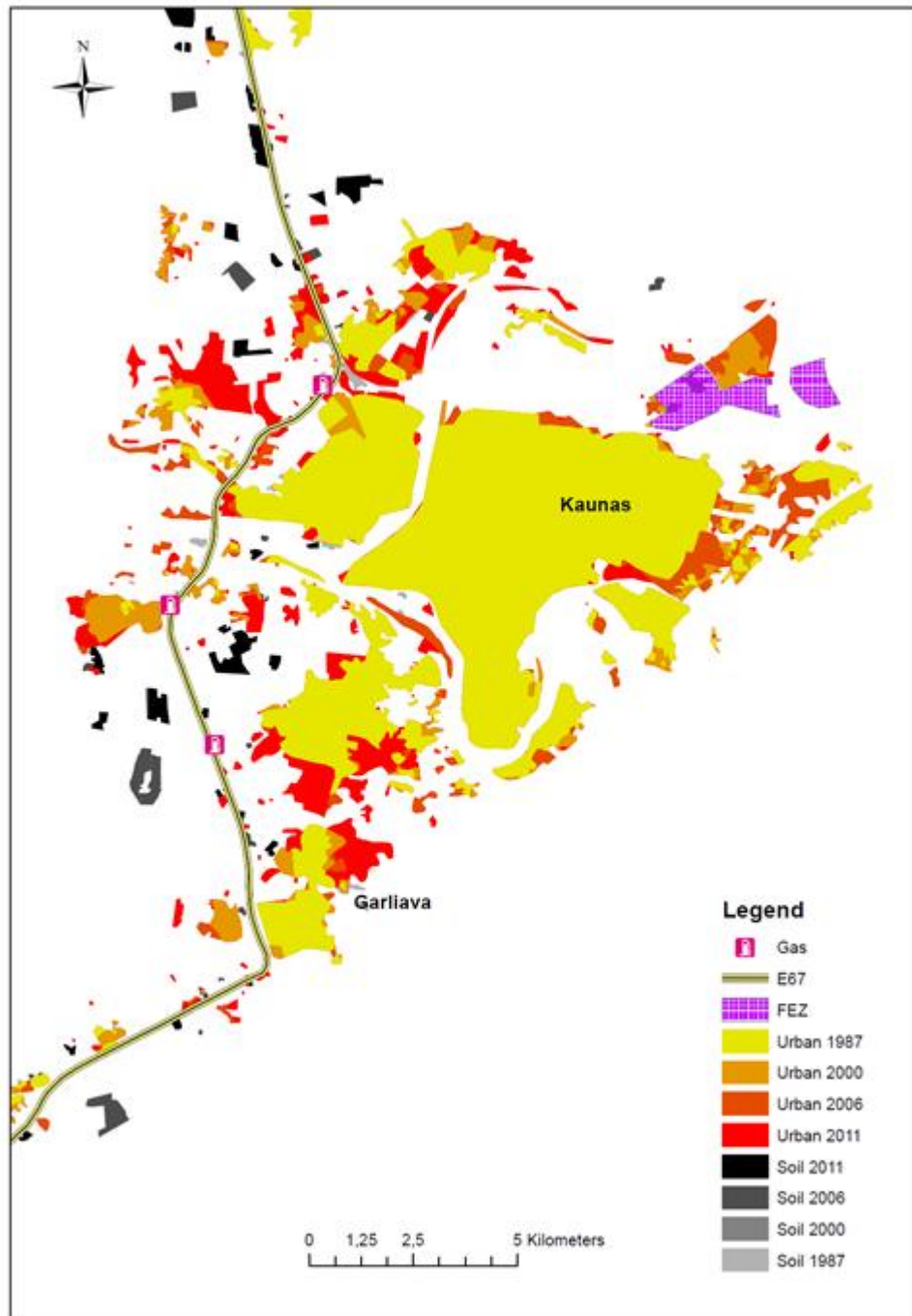
Figure 32: Urban growth of Kaunas (1987-2000-2006-2011)
