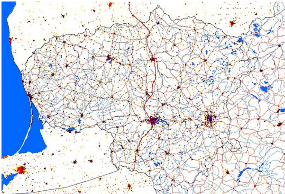
Figure 30: Local growth of urbanization within the Via Baltica
