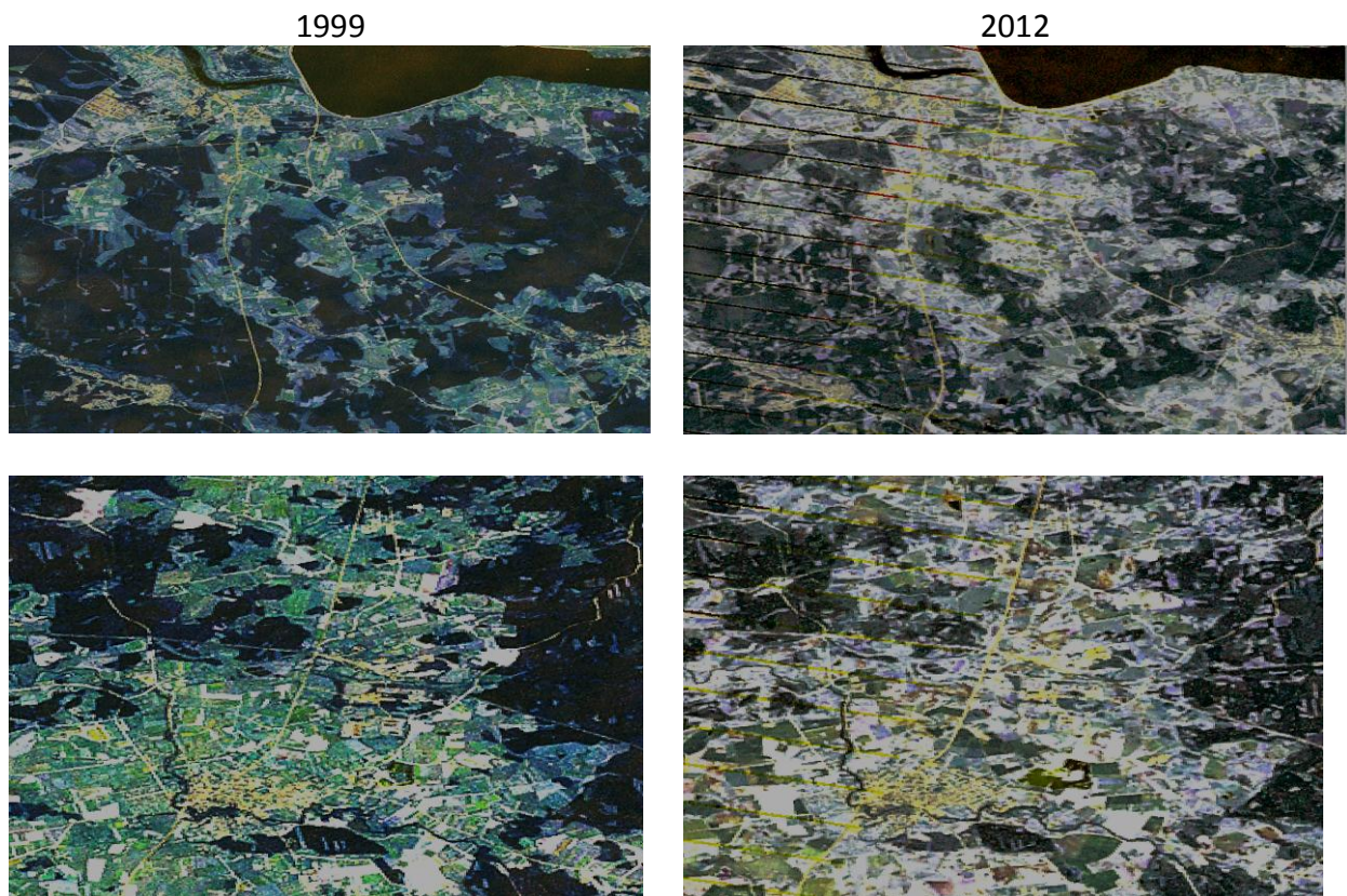
Figure 21: Riga's suburban places within the Via Baltica
