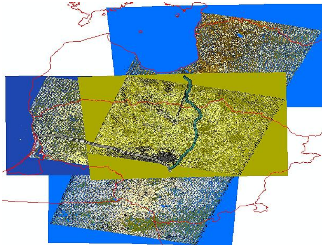
Figure 16: Example of the region of interest (Via Baltica and Kaunas-Klaipeda highway) (2012)
