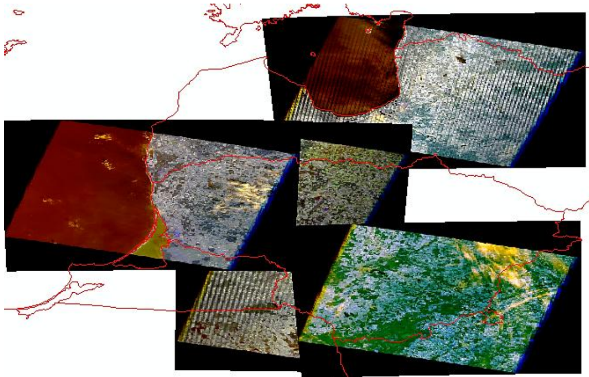
Figure 4: Example of Landsat mosaic on the region of interest (Riga-Kaunas-Klaipeda) in 2012
