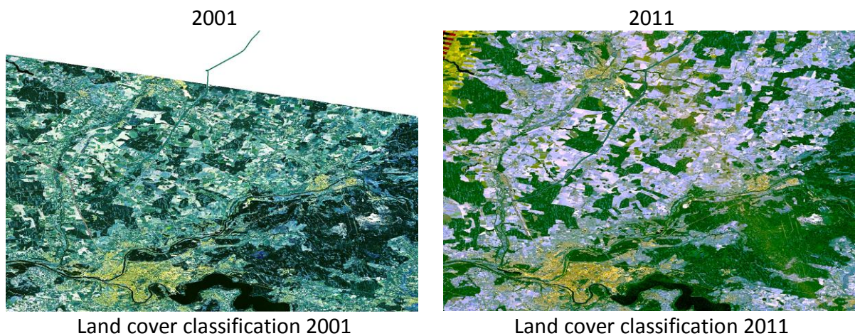
Figure 24: Urbanization of Kaunas region near the Via Baltica
