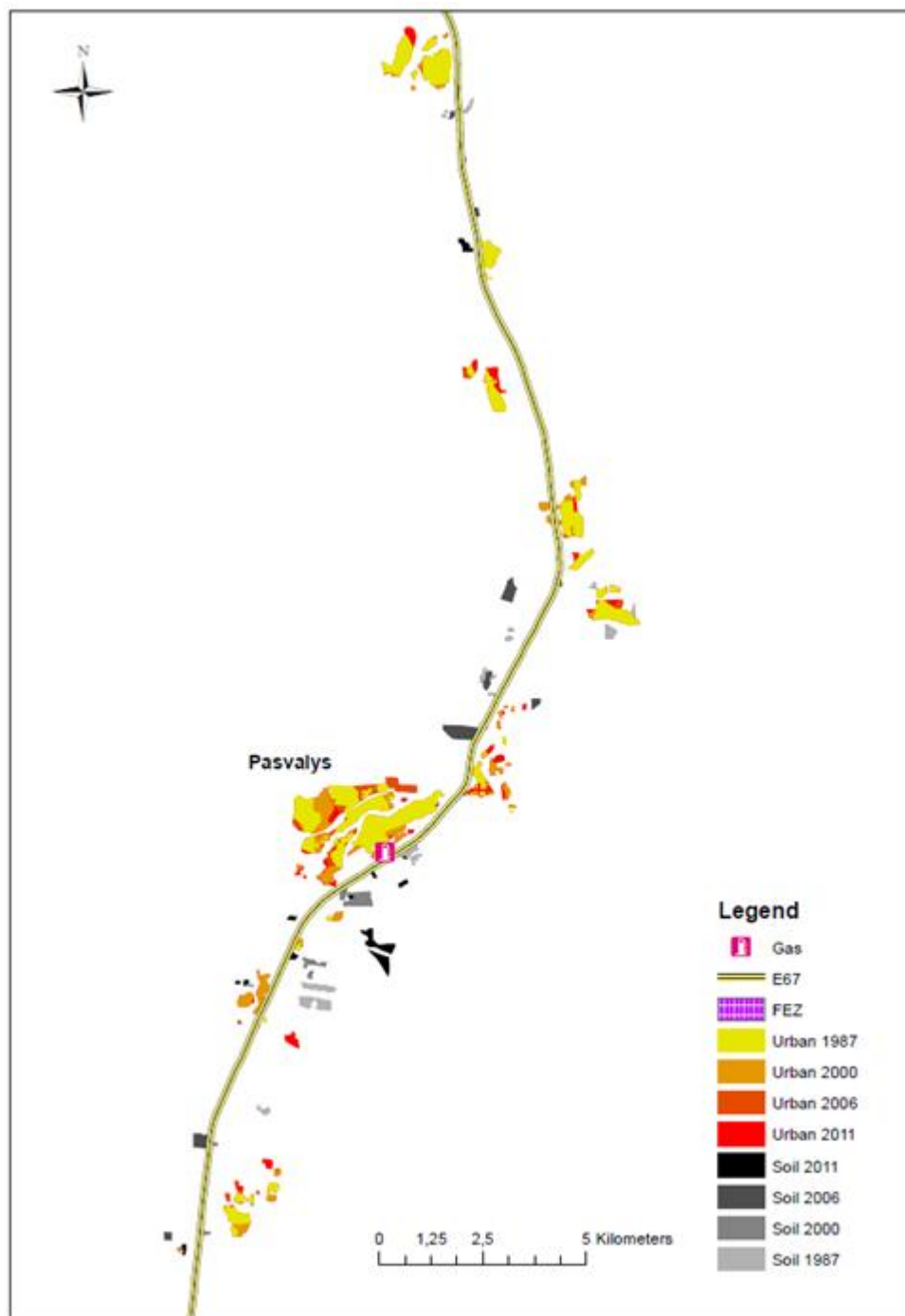
Figure 27: Urban distribution of Pasvalys region in 2011
