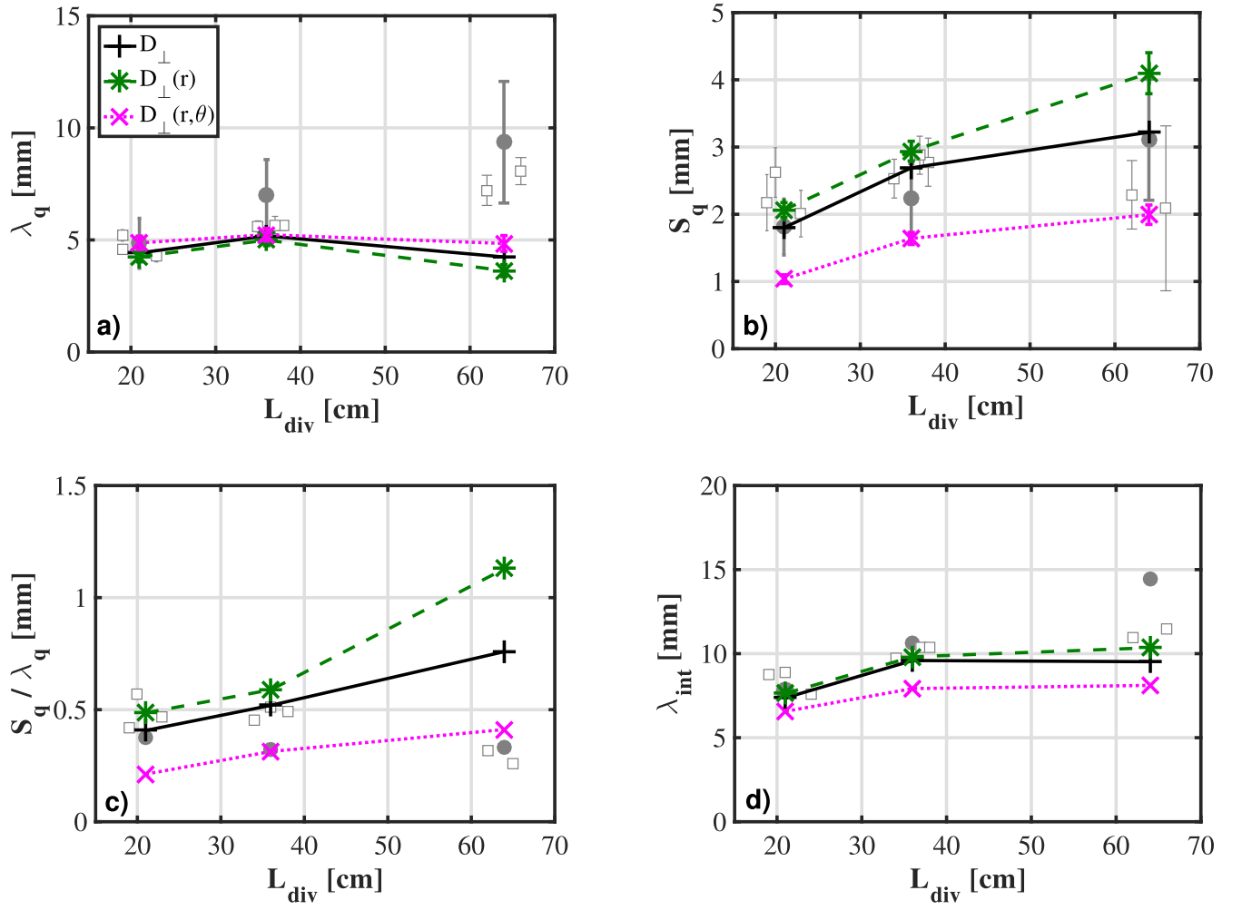
Figure 9. Numerical results of (a) \lambda_q , (b) S_q , (c) S_q/\lambda_q and d) \lambda_{\text{int}} as a function of L_{\text{div}} for constant D_{\perp} (solid black line), D_{\perp}(r) (dashed green line), D_{\perp}(r, \theta) (dotted magenta line). Grey markers refer to experimental data shown in figure 7.
