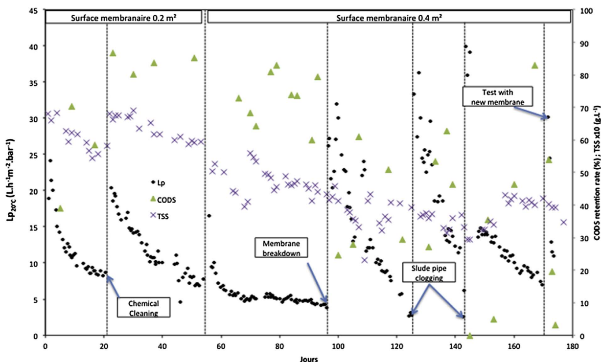
Fig. 8. Evolution of the membrane permeability, the supernatant \text{COD} retention rate and TSS ( \times 10 ) during the 2nd experimental campaign (sMBRE).
