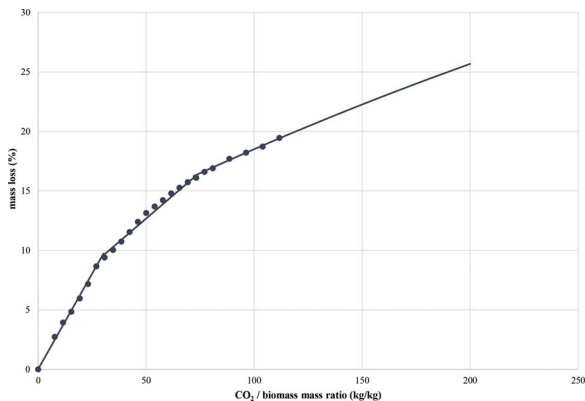
Fig. 7. JC SC-CO 2 extraction curve published by Micic et al. and modelled with BIC model (extraction of type B, P = 30 MPa and T = 323 K).
