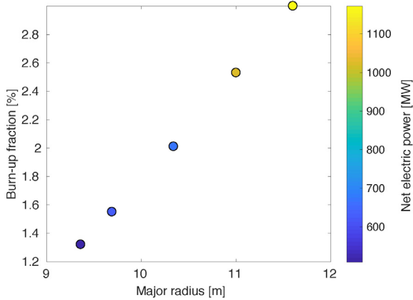
Fig. 4. Smallest DEMO1-like reactor for a number of different burn-up targets. Corresponding net electric power as a colorscale.
