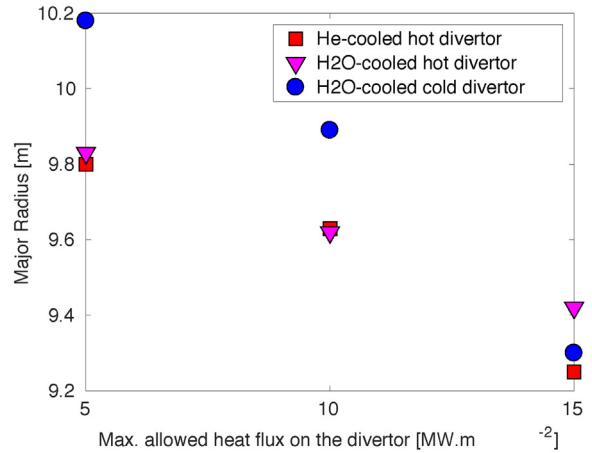
Fig. 5. Smallest DEMO1-like reactor for a range of divertor coolant scenarios.
