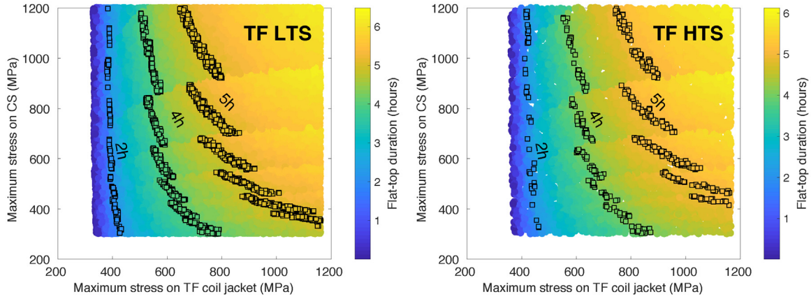
Fig. 2. Evolution of burn duration by varying \sigma_{max,TF} . Left: LTS. Right: HTS.
