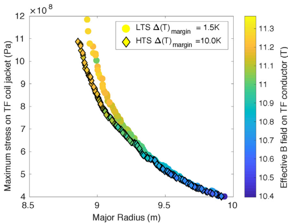
Fig. 1. Smallest DEMO1-like reactor for a range of maximum stresses allowed on the TF steel, with corresponding maximum field on the TF conductor.
