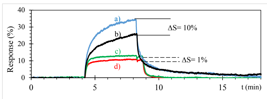
Figure 2. Sensor response for 500 ppb of BTEX without membrane SF a) in dry air b) in wet air (50% RH) and with membrane SF c) in dry air, d) in wet air (50% RH)
