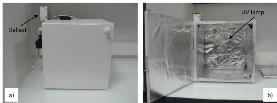
Fig. 1. Home-made UV irradiation chamber, lined inside of aluminum foil, equipped with UV lamp (after light bulb was removed) and a ballast for lamp operating. (a) Outside view, (b) Inside view.
