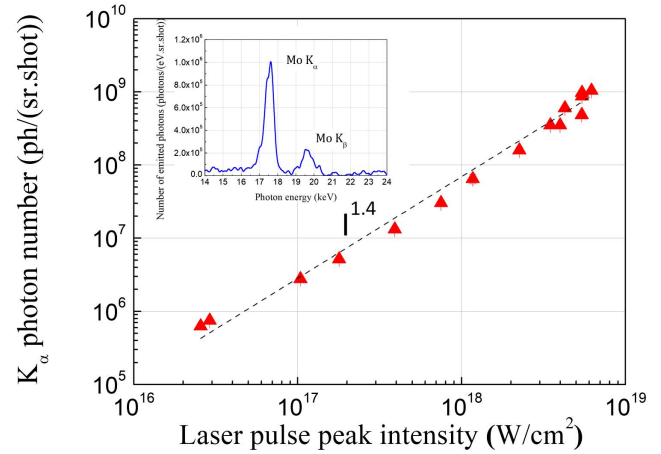
Fig. 1. K_\alpha production as a function of the laser peak intensity. The error bar associated with each value is given by the standard deviation calculated from three independent measurements of the K_\alpha photon production. The inset shows an absolute energy spectrum of the Mo x-ray emission obtained with the x-ray CCD camera for the laser intensity of I = 3 \times 10^{17} \text{W}/\text{cm}^2 .
