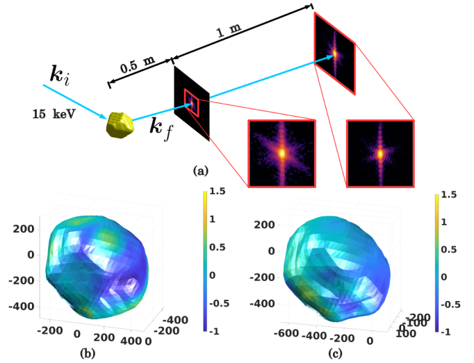
FIG. 6. (a) Experimental schematic for mock high-energy BCDI measurement. (b) Gold nanocrystal from modified phase retrieval acting on signal collected at a distance of 0.5 m [isosurface colored by phase (rad)]. (c) The same nanocrystal from conventional phase retrieval acting on signal collected at 1.5 m. The axis units in (b) and (c) are in nanometers.
