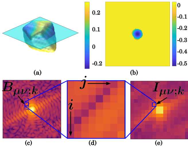
FIG. 2. (a) A simulated complex-valued 3D object ( 128 \times 128 \times 70 pixels) with surface phases, with the color scale in units of radians. (b) A 128 \times 128 -pixel slice depicting the phase through the middle of the object in (a). (c) High-resolution diffraction pattern representing the k th 2D slice of the 3D intensity pattern (in simulated photon counts) corresponding to the object in (a). A contiguous 8 \times 8 block in this pattern is indexed by (\mu, \nu) , along with neighboring blocks (\mu \pm 1, \nu) . (d) Zoom-in of the block in (c). (e) Binned diffraction pattern ( 16 \times 16 ) showing a pixel whose intensity is the sum of those in the block B_{\mu\nu k} .
