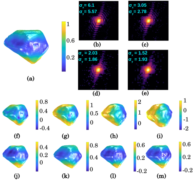
FIG. 3. (a) Isosurface plot of a synthetic particle reconstructed with conventional phase retrieval ( \alpha = 1 ), which we use as a ground truth for comparison. (b)–(e) Central slices through binned diffraction signals (simulated photon counts) for \alpha = 2, 4, 6, 8 , respectively, with steadily degrading fringe visibility (including sampling rates \sigma_x, \sigma_y along the axes of the imaging plane). (f)–(i) Isosurface plots of synthetic particles recovered using conventional phase retrieval on binned noisy signals with \alpha = 2, 4, 6, 8 . (j)–(m) Isosurface plots of synthetic particles recovered using modified phase retrieval on binned noisy signals with \alpha = 2, 4, 6, 8 show much better agreement with (a). All the color bars denote the phase expressed in radians. The pixelation in the final reconstructions was removed by Gaussian kernel smoothing and the isosurfaces were plotted at a value of 0.5 of the maximum object amplitude.
