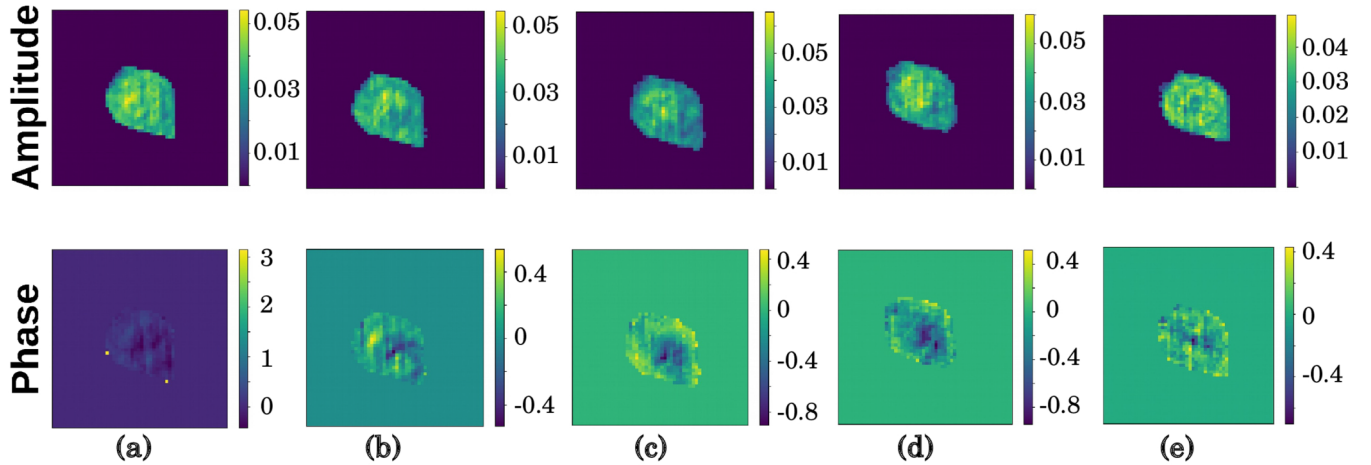
FIG. 4. (a) Amplitude and phase cross sections of the reconstructed crystal shown in Fig. 3(a), from conventional phase retrieval applied to unbinned diffraction (prior to Gaussian filtering). (b)–(e) Slices from the reconstructions corresponding to \alpha = 2, 4, 6, 8 . The amplitude is expressed in arbitrary units, while the phase is expressed in radians. The central dip in the phase is discernible in all reconstructions.
