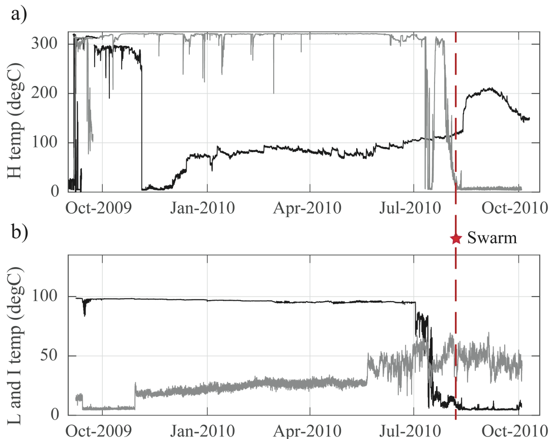
Figure 3: Temperature records for the period Oct. 2009- Oct. 2010. a) Temperature data from two HT sensors deployed on black smoker chimneys at Eiffel Tower vent (TE-V02-090905-101003-HW0010B in gray) and Aisics vent (TE-AIS-090923-101010-HN29016b in black). b) Temperature data from a LT sensor deployed on a diffuse crack at Eiffel Tower vent (TE-C02-090907-101003-LW00003, black), and at Montsegur vent (MS-C02-090907-101004-LW00001, gray). The red star and dashed line represent a seismic swarm recorded through Ocean Bottom Seismometer (OBS) network deployed during the same period of time around LSHF [Crawford et al, 2013].
