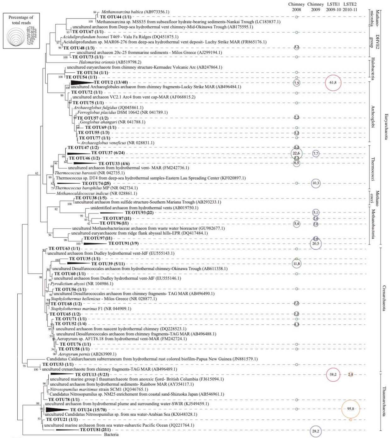
Figure 5: Phylogenetic relationships among the archaeal 16S rRNA gene sequences of representative OTUs of the four samples. Sequences from this study are designed by the prefix “TE”. The corresponding number of OTU/sequences for each representative OTU is indicated in bracket. The circle size figures the percentage represented by each OTU with respect to the total number of sequences for each sample. The closest NCBI sequences are presented with their GenBank accession numbers. The tree was constructed by Maximum Likelihood method.
