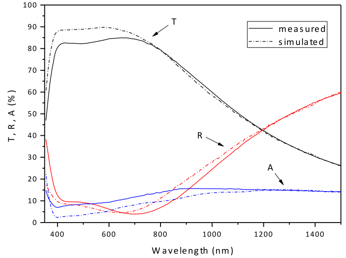
Fig. 2. Simulated and measured transmittance ( T ), reflectance ( R ) and absorptance ( A ) for Glass/ZnS (40 nm)/Ag (10 nm)/ \text{TiO}_x (35 nm).
