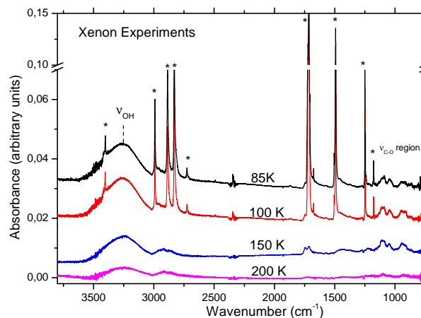
Figure 5. Infrared spectrum of the solid film obtained after xenon desorption (85 K) from the sample recorded during the warming from 85 to 200 K (4 K min -1 ). Bands labeled with stars are due to formaldehyde.
