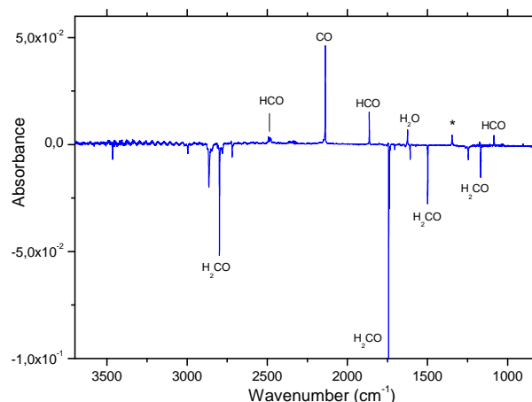
Figure 1. Difference infrared spectrum after VUV photolysis (30 min, \lambda > 120 nm) at 12 K in Ar matrix. Negative bands stand for H 2 CO, while positive bands stand for photo-products. Bands labeled with stars refer to unknown species.
