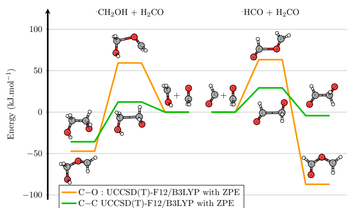
Figure 9. Left: \text{·CH}_2\text{OH} + \text{H}_2\text{CO} reaction paths for the C–C bond formation (green) and C–O bond formation (yellow) in the initiation steps (5) and (6). Right: \text{·HCO} + \text{H}_2\text{CO} reaction paths for the C–C bond formation (green) and C–O bond formation (yellow) in the initiation steps (3) and (4) respectively (See text).
