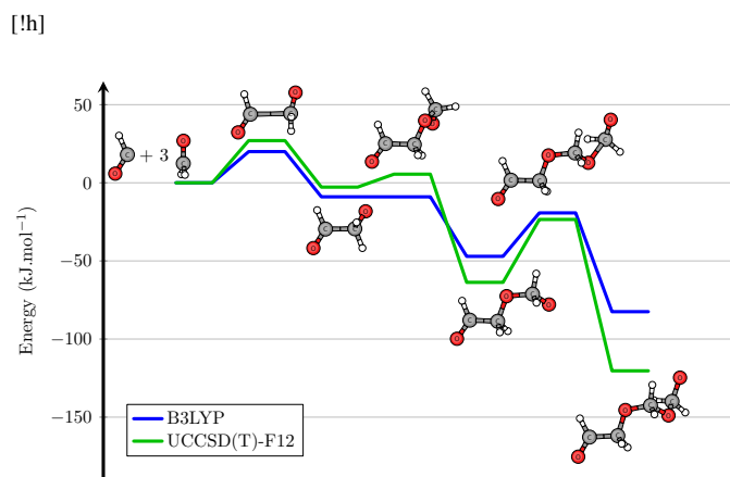
Figure 10. Reaction path of the initiation step (C–C bond formation) and the first two propagation steps for reaction (1) (See text).
