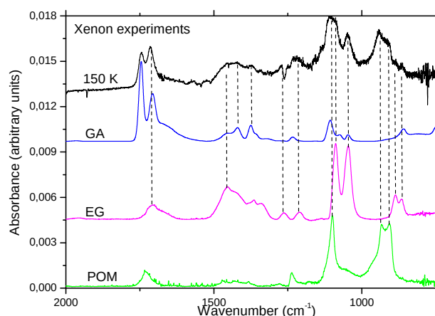
Figure 6. Infrared spectrum of the solid film recorded at 150 K after Xenon desorption from the sample at 85 K. It is compared to reference spectra of polyoxymethylene, ethylene glycol, and glycolaldehyde. See experimental part for details.
