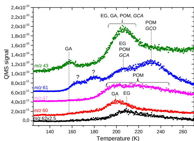
Figure 7. Temperature Programmed Desorption (TPD) spectra of the solid film formed after rare gas desorption step of the photolysis at 12 K ( \lambda > 120 nm, 30 min) of \text{H}_2\text{CO}/\text{Ar} = 2/1000 matrix. m/z 43: \text{CHOCH}_2^+ ; m/z 47: \text{HOCH}_2\text{O}^+ ; m/z 60: \text{HOCH}_2\text{CHO}^+ ; m/z 61: \text{HOCH}_2\text{CH}_2\text{O}^+/\text{HOCH}_2\text{OCH}_2^+ ; m/z 62: \text{HOCH}_2\text{CH}_2\text{OH}^+ . GA: m/z 61, 43; EG: m/z 62, 61, 43; POM: m/z 61, 47, 43; GCA: m/z 61, 43; GCO: m/z 61 43. GCA and GCO detections are only tentative.
