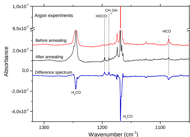
Figure 2. Infrared difference spectrum showing the effect of annealing at 30 K after the VUV photolysis ( \lambda > 120 nm, 30 min) of formaldehyde in Ar matrix. Positive bands relates to formed species and negatives bands to consumed species
