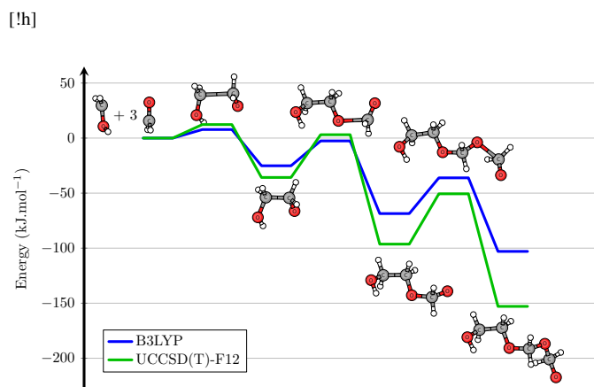
Figure 11. Reaction path of the initiation step (C–C bond formation) and the first two propagation steps for reaction (2) (See text).
