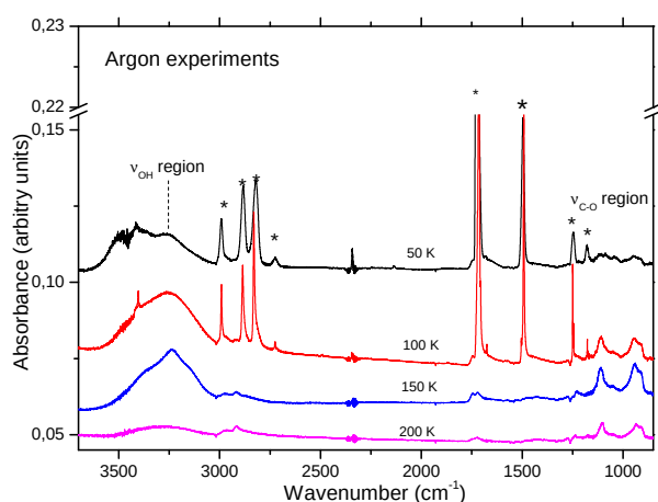
Figure 3. Infrared spectrum of the solid film obtained after argon desorption (35 K) from the sample recorded during the warming from 50 to 200 K (4 K min -1 ). Bands labeled with stars are due to formaldehyde.
