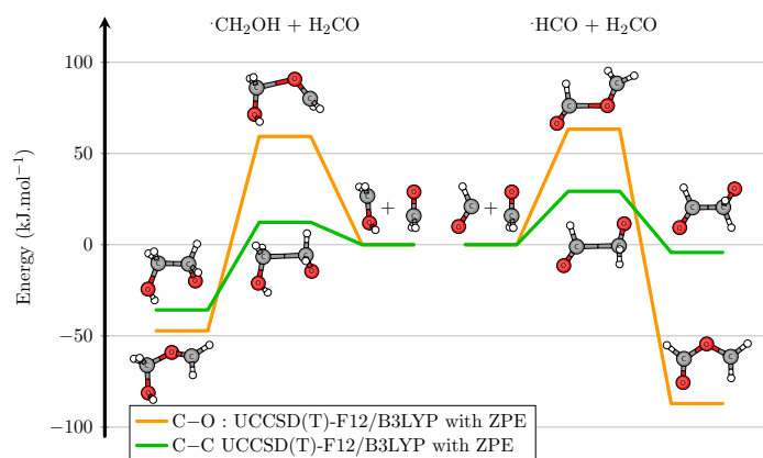
Figure 9. Left: \cdot\text{CH}_2\text{OH} + \text{H}_2\text{CO} reaction paths for the C–C bond formation (green) and C–O bond formation (yellow) in the initiation steps (5) and (6). Right: \cdot\text{HCO} + \text{H}_2\text{CO} reaction paths for the C–C bond formation (green) and C–O bond formation (yellow) in the initiation steps (3) and (4) respectively (See text).
