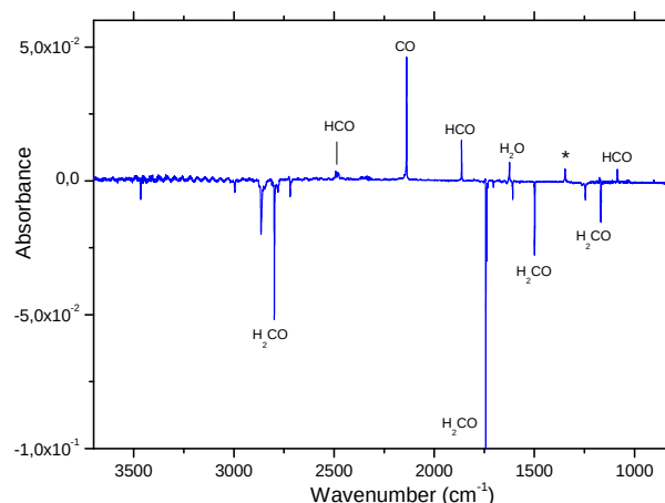
Figure 1. Difference infrared spectrum after VUV photolysis (30 min, \lambda > 120 nm) at 12 K in Ar matrix. Negative bands stand for \text{H}_2\text{CO} , while positive bands stand for photo-products. Bands labeled with stars refer to unknown species.
