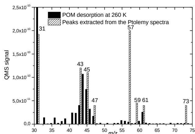
Figure 12. Mass spectrum of POM recorded at 260 K compared with extracted peaks from the Ptolemy spectra. m/z 44 is related to \text{CO}_2 contamination.
