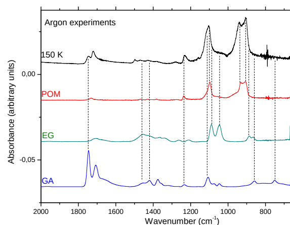
Figure 4. Infrared spectrum of the solid film recorded at 150 K after Ar desorption from the sample at 35 K. It is compared to reference spectra of polyoxymethylene, ethylene glycol, and glycolaldehyde
