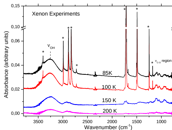
Figure 5. Infrared spectrum of the solid film obtained after xenon desorption (85 K) from the sample recorded during the warming from 85 to 200 K (4 K min -1 ). Bands labeled with stars are due to formaldehyde.
