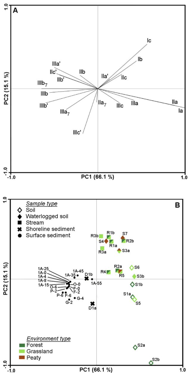
Fig. 4. Compositional analysis of brGDGT distributions from catchment and sediment samples. Compositional analysis based on the fractional abundances of the 18 brGDGTs in the surface samples (IIIa' was not considered) at Lake St Front including catchment soils and surface and sub-surface sediments (0–50 cm, n = 37 ). A. Scores of the brGDGT compounds on PC1 and PC2. B. Scores of the surface sediment (circles), waterlogged (filled diamonds), and other soil (open diamonds), stream (squares), and shoreline samples (crosses) along with their reference names (see Table 1). The environment of the samples has been identified as woodland (dark green), grassland (light green) or peaty (brown). (For interpretation of the references to colour in this figure legend, the reader is referred to the web version of this article.)
