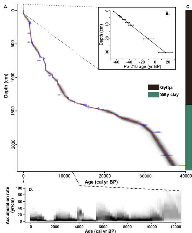
Fig. 2. Age-depth model and accumulation rate for the Lake St Front sediment core. A. Age-depth model obtained with the Bacon software (Blaauw and Christen, 2011). The grey dotted lines indicate the 95% confidence limits and the red dotted line shows the weighted mean ages for each depth. The shaded area indicates the density of individual age-depth iterations. The calibrated age range of ^{14}\text{C} -dated samples is indicated in blue. B. ^{210}\text{Pb} ages for the upper 30 cm of the core. C. Lithology of the sedimentary sequence of Lake St Front. D. Accumulation rate for the last 12,000 years cal BP obtained with the Bacon software (Blaauw and Christen, 2011). The shaded area indicates the probability density. (For interpretation of the references to colour in this figure legend, the reader is referred to the web version of this article.)
