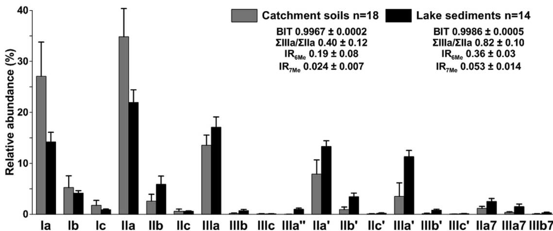
Fig. 3. Modern brGDGT distributions. Average fractional abundance of each brGDGT in catchment soils and streams ( n = 18 , grey) and lake sediments (0–10 cm, n = 14 , black). Average BIT index values, as well as \Sigma IIIa/\Sigma IIa and isomer ratios for each group are provided with 1\sigma standard deviation.
