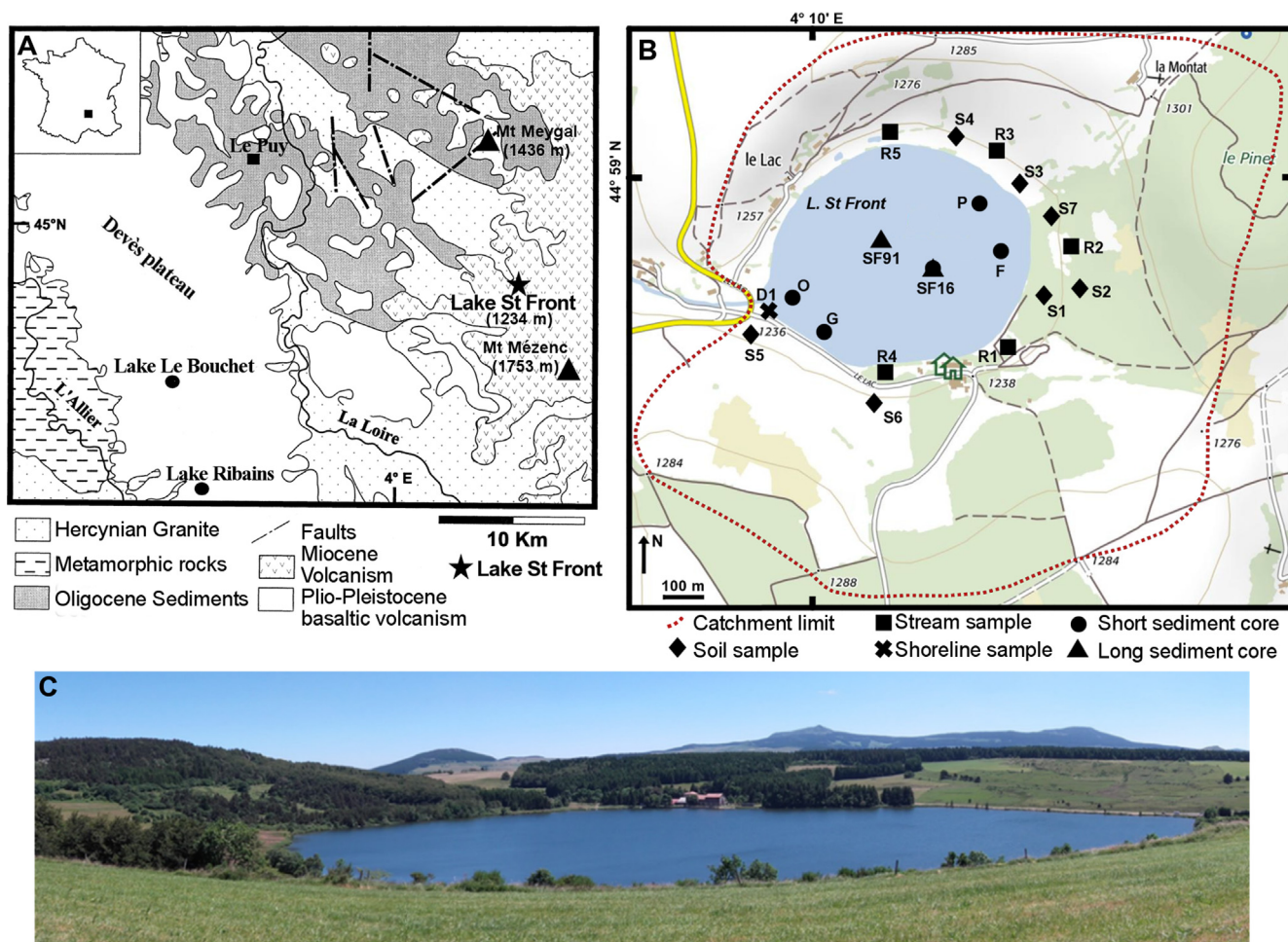
Fig. 1. Lake St Front with locations of the soil, stream, and sediment samples. A. Simplified geologic map of the Devès and Meygal-Mézenc plateaux forming the Velay region showing the location of Lake St Front with its altitude and the relevant archives at a regional scale (modified from Stockhausen and Thouveny, 1999). B. Map of Lake St Front and sampling locations for the deep sediment cores (triangles), shallow interface sediment cores (circles), soils (diamonds), streams (squares), and shoreline (crosses) along with their reference names. The catchment area is enclosed by the dotted dark red line and the woodland area is shaded in green. This topographic map was adapted from an original map provided by the Institut national de l'information géographique et forestière (IGN). C. Picture of the lake and its catchment area. (For interpretation of the references to colour in this figure legend, the reader is referred to the web version of this article.)
