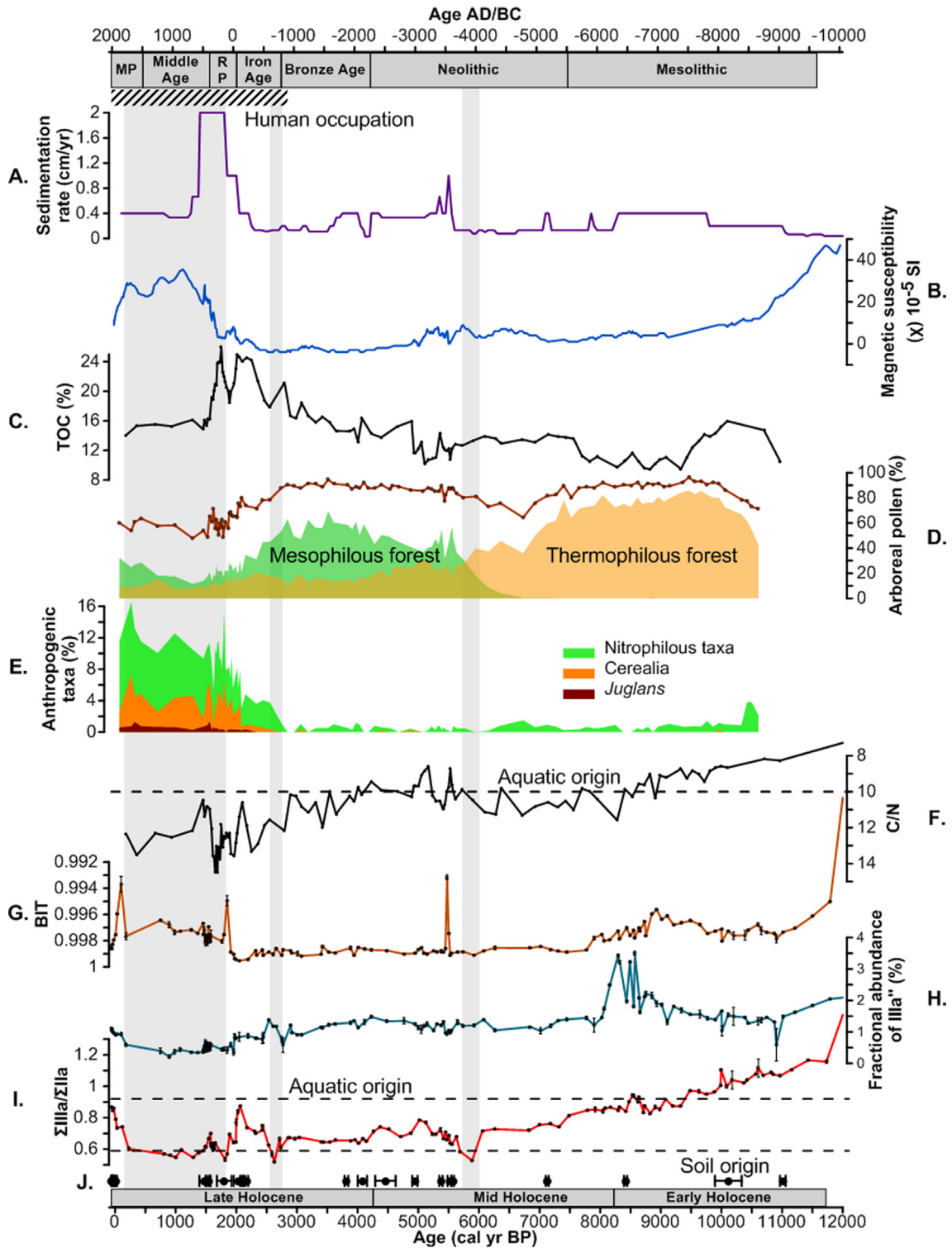
Fig. 5. Sedimentological, geochemical, and palynological evolution of the Holocene recorded at Lake St Front. A. Simplified sedimentation rate obtained from the Bacon program. B. Magnetic susceptibility. C. Total Organic Carbon (TOC, Rhoujjati, 1995 ). D. Percentage of arboreal pollen (brown curve) and percentages of pollen from thermophilous (beige area, sum of Acer , Hedera , Ilex , Lonicera , Ostrya , deciduous Quercus , Quercus ilex t., Pistacia , Sambucus , Sorbus , Tilia , Ulmus , Viburnum , Viscum ) and mesophilous (green area, sum of Abies , Carpinus , Fagus ) tree pollen. E. Cumulative percentages of pollen of nitrophilous taxa (light green area, Plantago lanceolata , P. major , Rumex , Chenopodiaceae , Urtica ), cereals (orange area, Cerealia , Secale ), and Juglans (burgundy area). F. C/N ratio ( Rhoujjati, 1995 ); note that the axis has been reversed for improved readability. The dashed line represents the upper limit of production in the aquatic realm. G. BIT index with analytical errors ( 1\sigma values); note that the axis has been reversed. H. Fractional abundance of Illa'' with analytical errors ( 1\sigma values). I. \Sigma IIIa/\Sigma IIa ratio (red curve) with analytical errors ( 1\sigma values). The dashed lines represent the upper limit of production in the terrestrial realm and the lower limit of production in the aquatic realm defined by Xiao et al. (2016) . J. ^{14}C calibrated ages and ^{210}Pb dates. Shaded rectangles highlight the periods when \Sigma IIIa/\Sigma IIa values are below the upper limit for soil origin. The period of permanent human occupation is marked by a hatched symbol. RP: Roman Period, MP: Modern Period. (For interpretation of the references to colour in this figure legend, the reader is referred to the web version of this article.)
